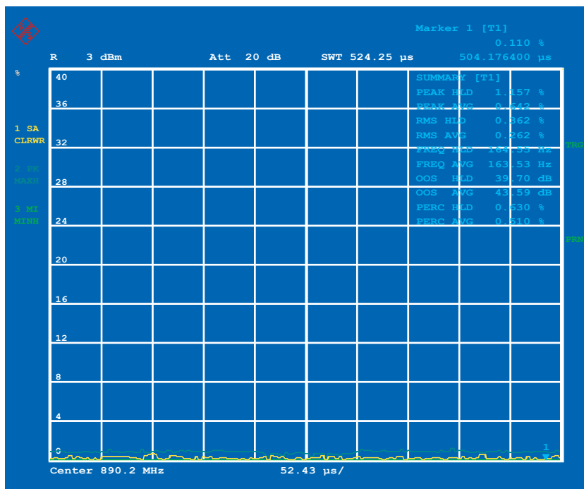
Measurement of modulation accuracy on EDGE burst.
