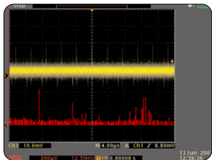
► Look for unintentional circuit noise with the TDS3000B Series' FFT capability.
