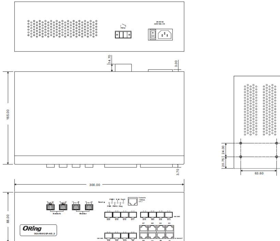
Wall-Mounting Measurement (Unit = mm)
