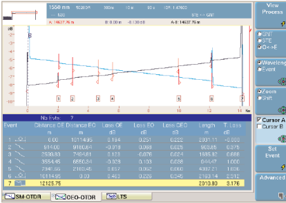
Figure 3 Bidirectional OTDR measurement
