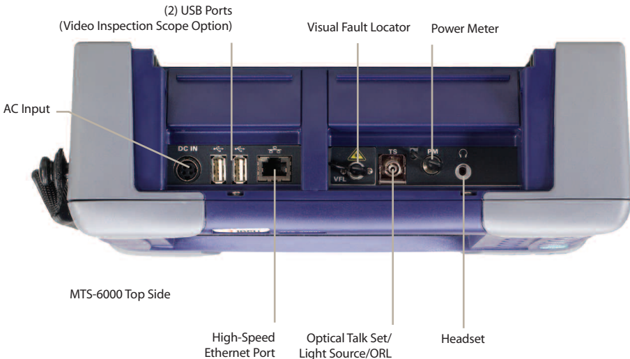
MTS-6000 Front Panel
