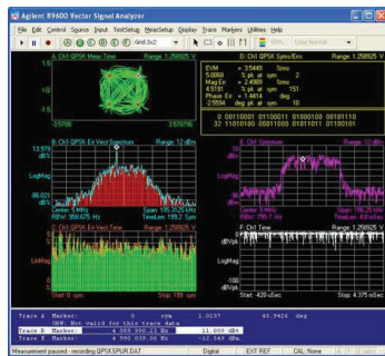
Use vector signal analysis software to see FFT-based spectrum analysis.
