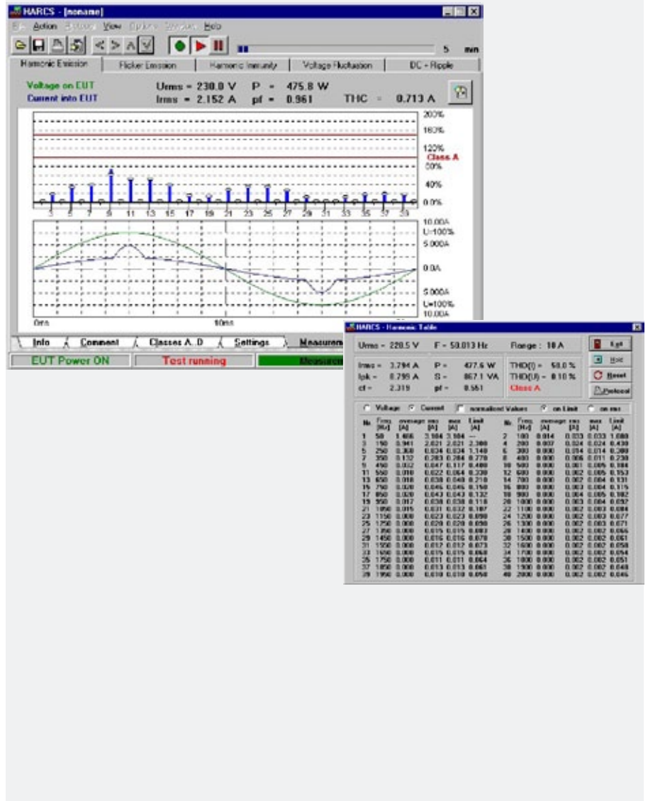
Display of single phase harmonic voltage and current (left)
