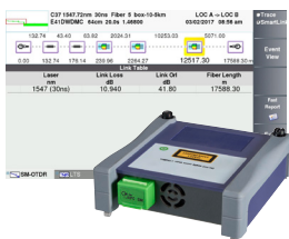
OneAdvisor-800
