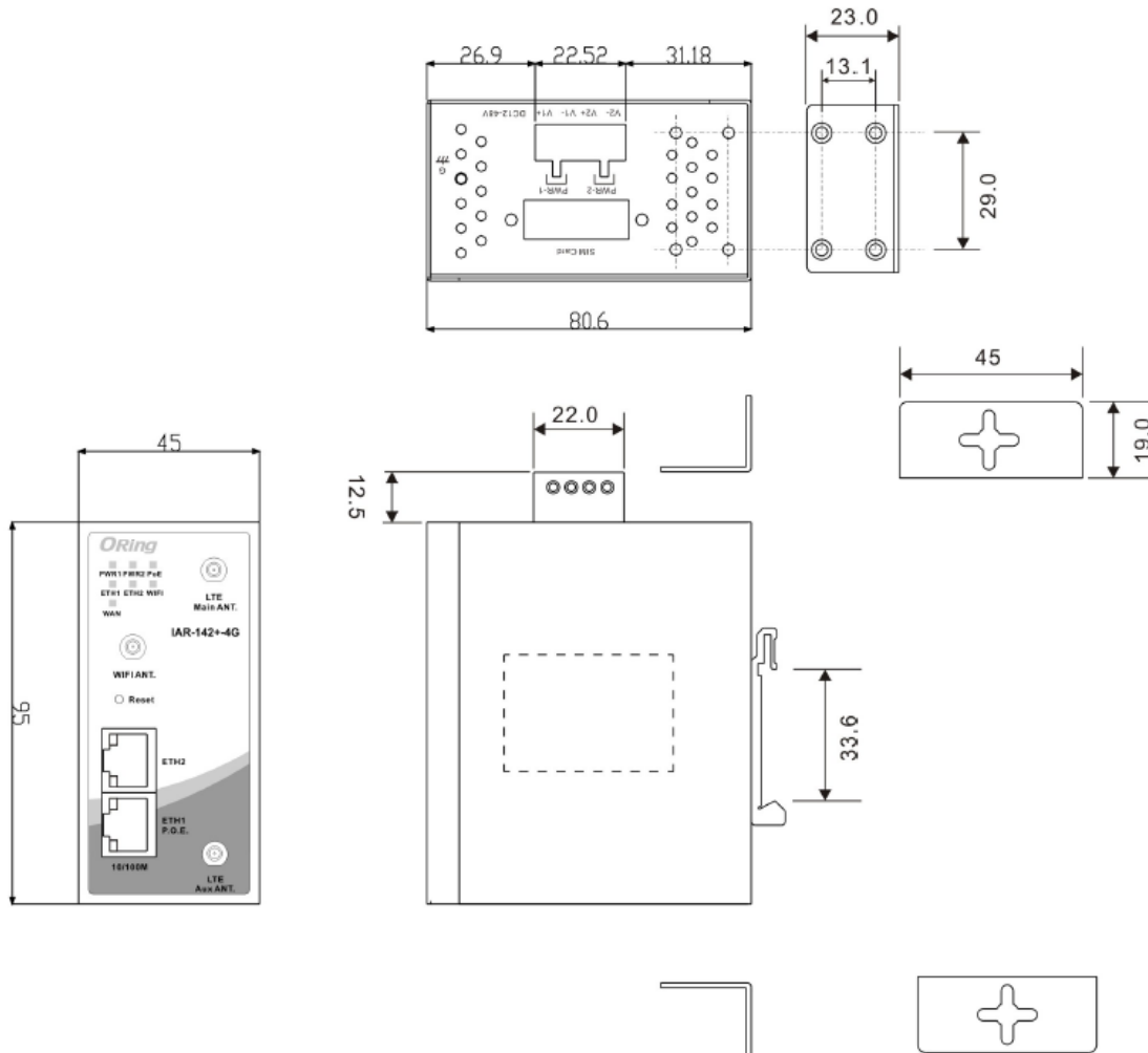
Wall-Mount Kit Measurement (Unit = mm)
