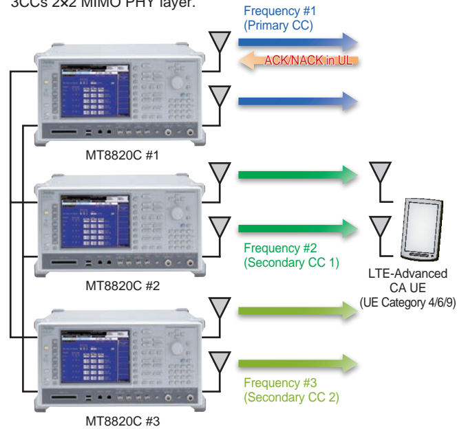
Sample MT8820C connection
