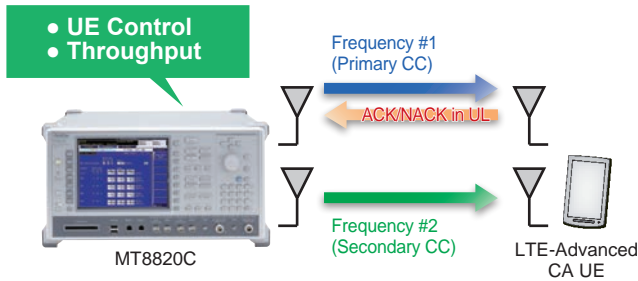
MT8820C Connection Example
