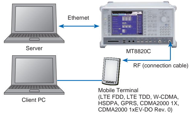
Sample MT8820C connection
