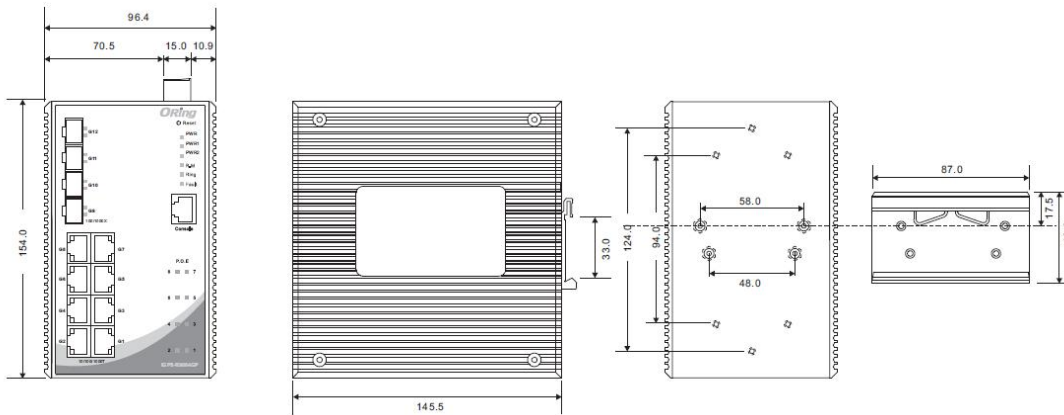
DIN-Rail Measurement (Unit = mm)
