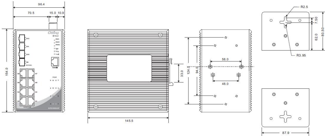
Wall-Mounting Measurement (Unit = mm)
