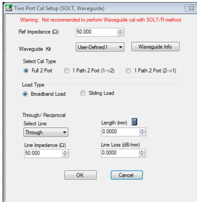
Figure 3-3. TWO PORT CAL SETUP (SOLT/R, WAVEGUIDE) Dialog Box
