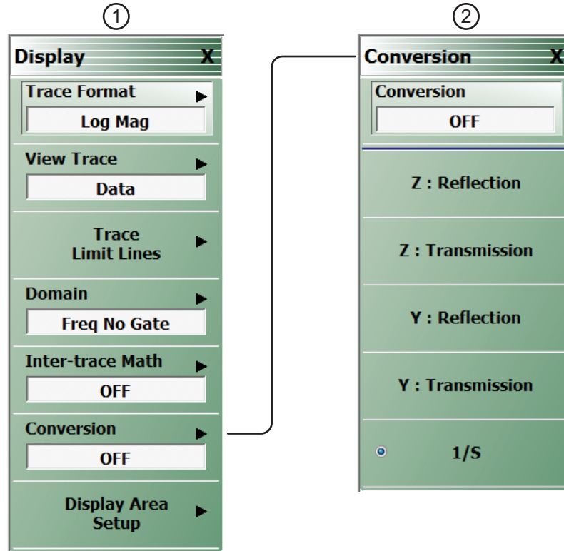
Figure 10-14. Conversion Control Menus
