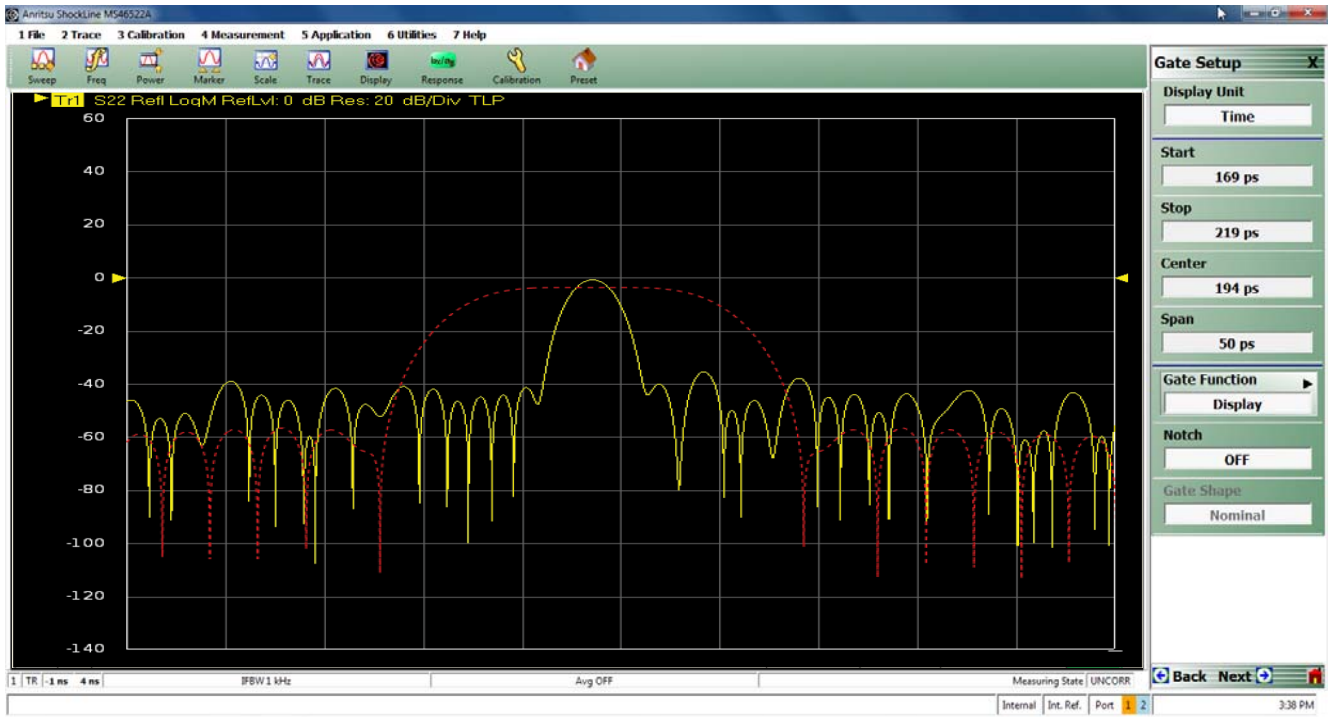
Figure 12-18. Gate in Display Mode Example
