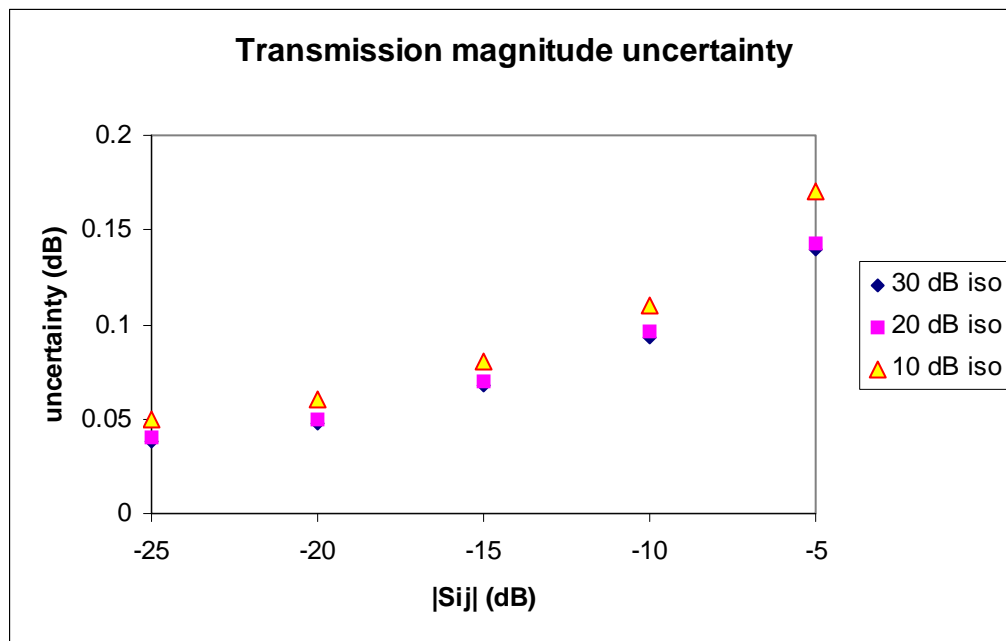
Figure 16-22. Transmission Magnitude Uncertainty
