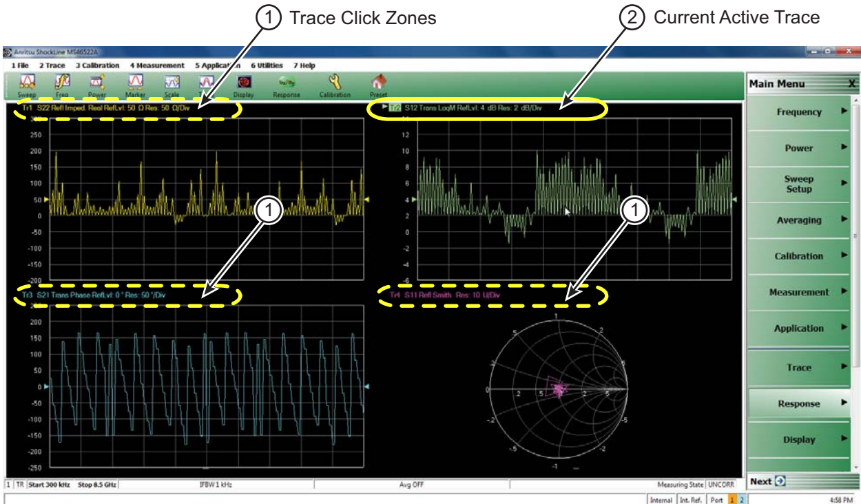
Figure 11-6. Trace Activate Click Zones
