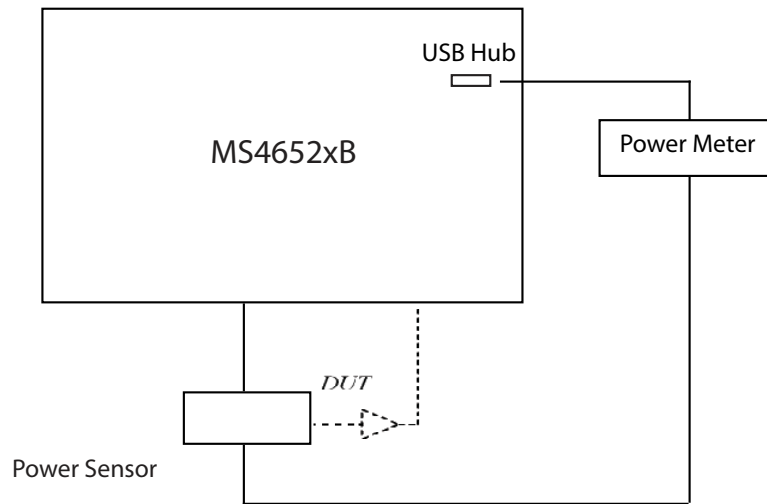
Figure 14-3. Power Calibration Setup
