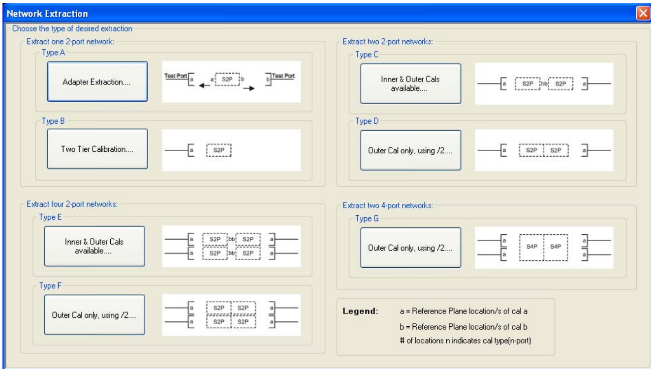
Figure 16-29.NETWORK EXTRACTION Dialog Box - Type Selection - 4-Port VNAs
