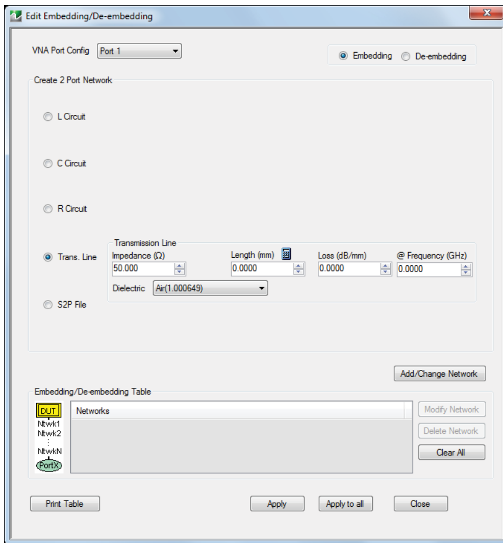
Figure 10-7. EDIT EMBEDDING/DE-EMBEDDING Dialog Box
