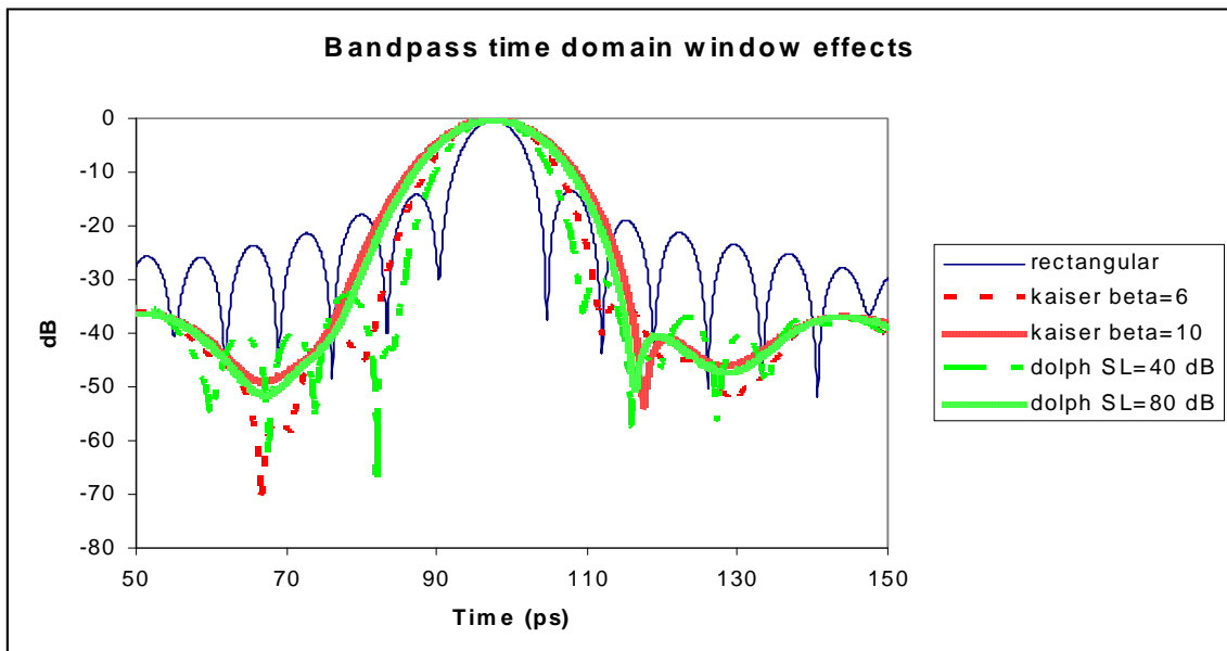
Figure 12-15. Window Effects in Bandpass Time Domain (advanced window types)
