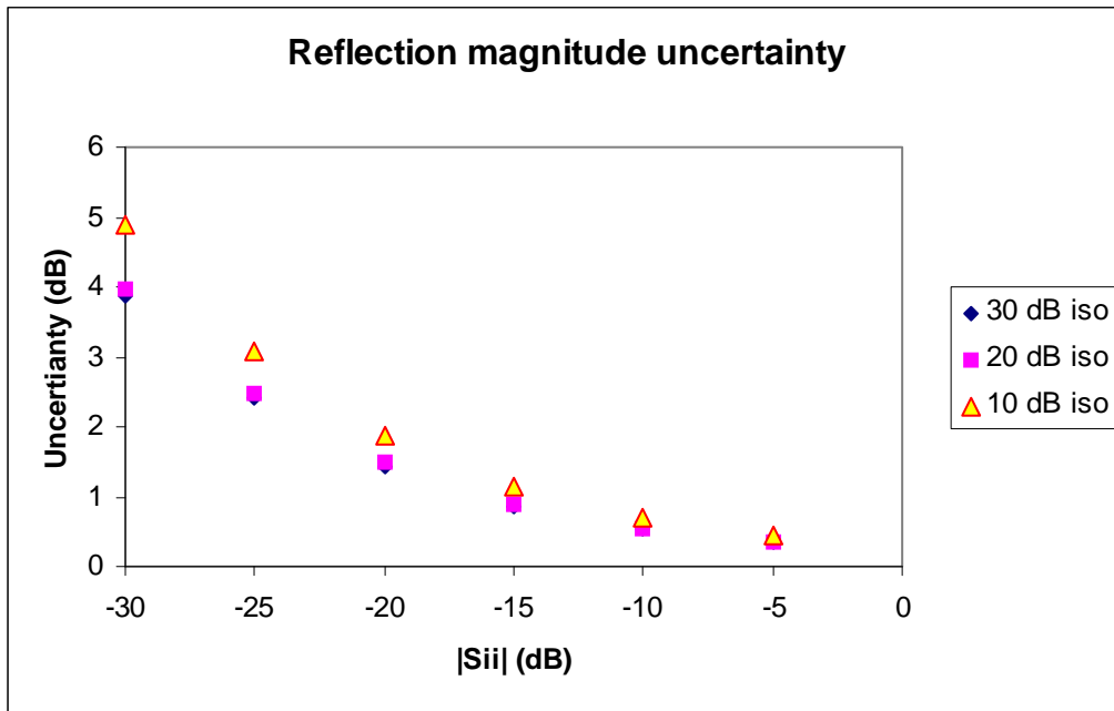
Figure 16-23. Reflection Magnitude Uncertainty
