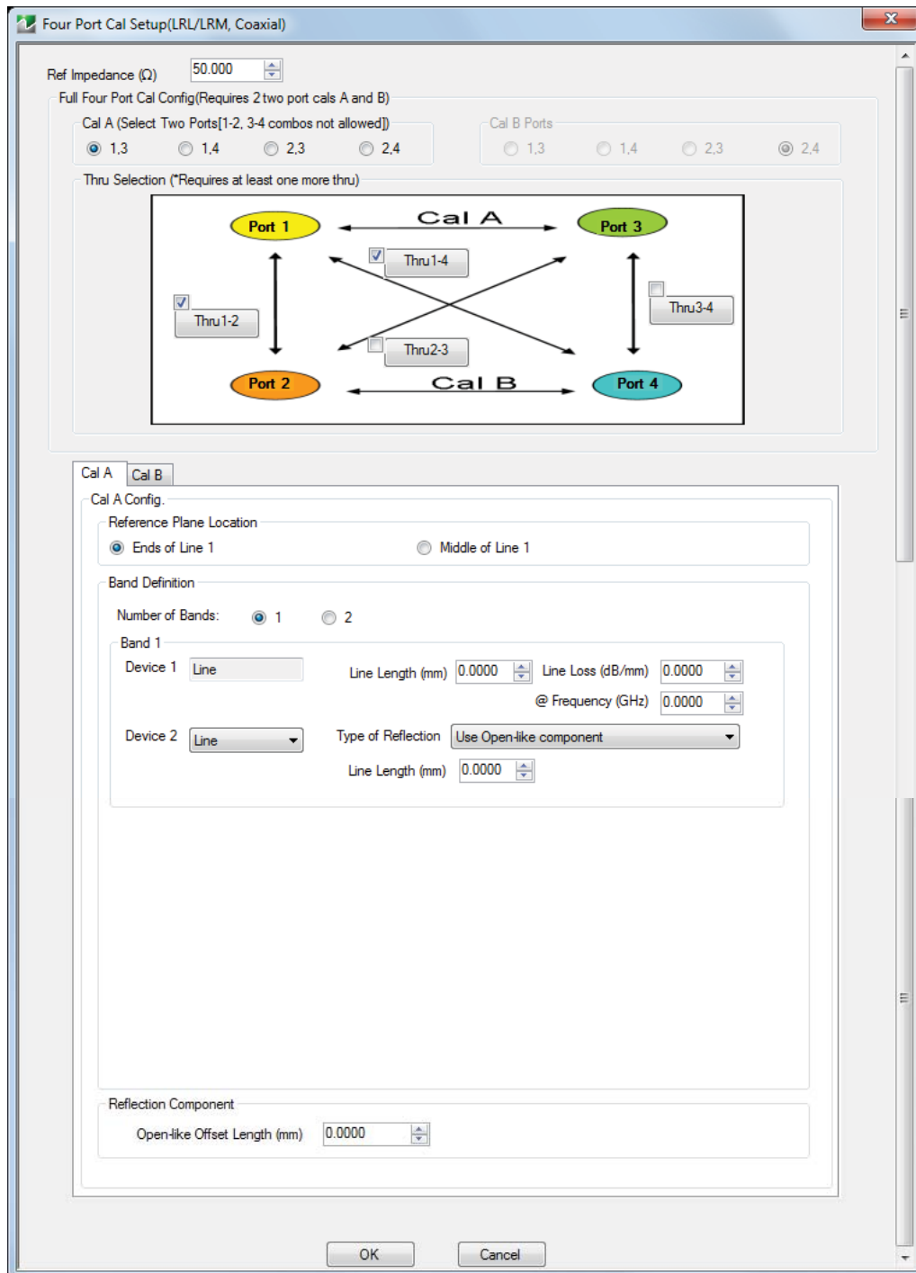
Figure 16-17. FOUR PORT CAL SETUP (LRL/LRM, COAXIAL) Dialog Box
