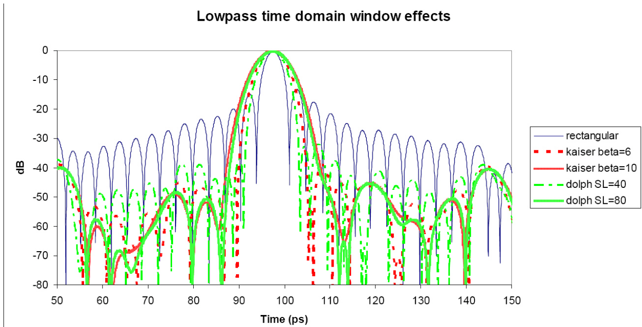
Figure 12-9. Effects of Window Shapes Plot with Advanced Windows Selection
