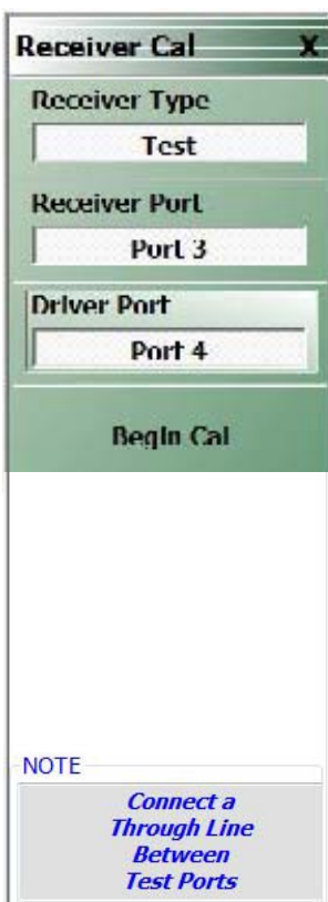
Figure 7-5. RECEIVER CAL (CALIBRATION) Menu
