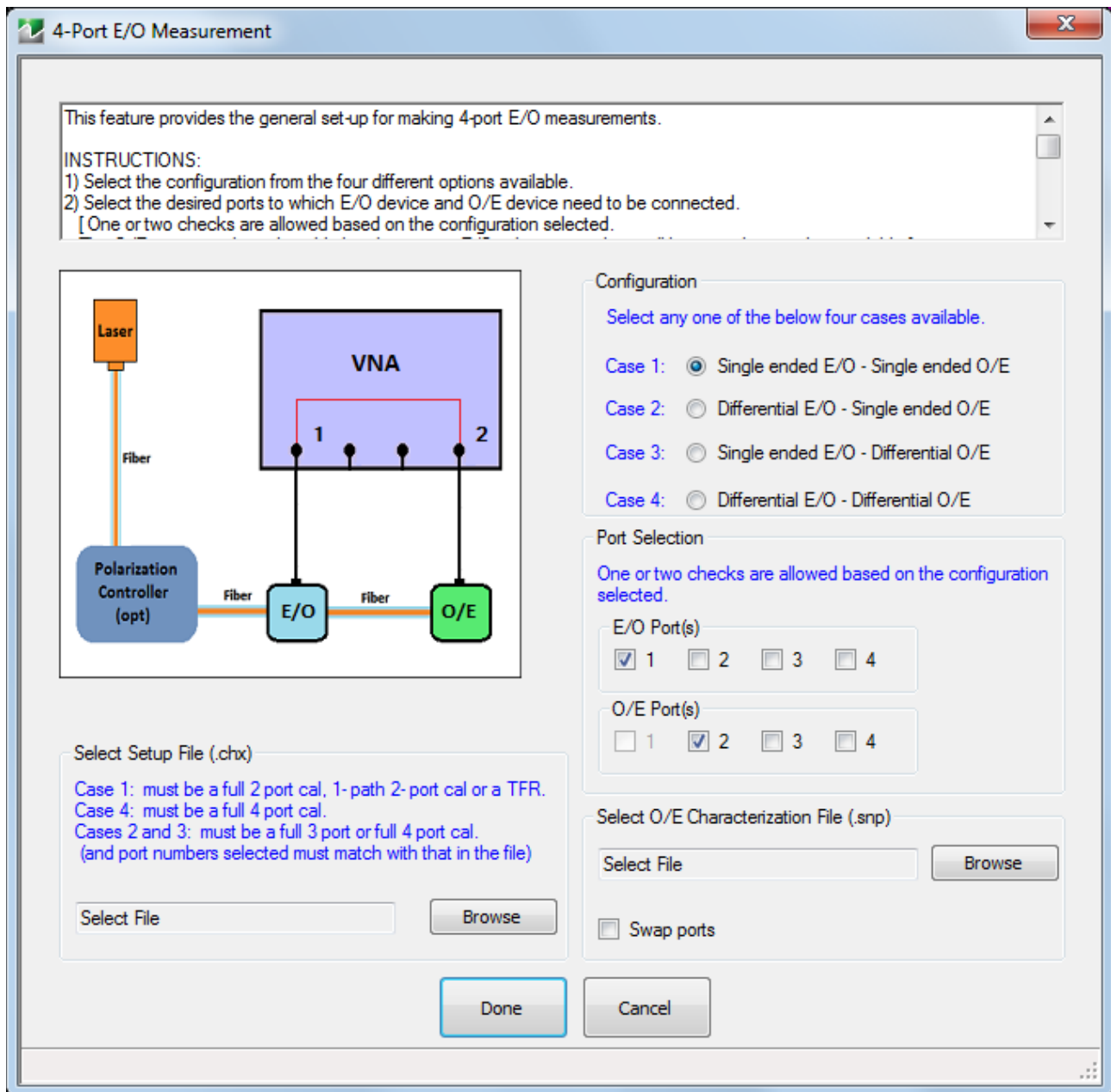
Figure 18-12. The dialog for 4-port E/O measurements is shown here.
