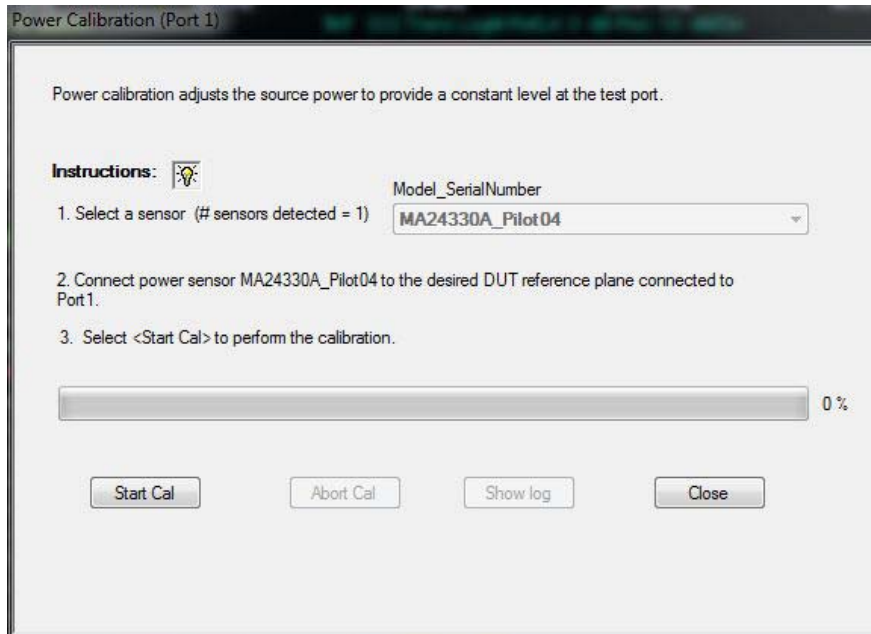
Figure 14-4. POWER CALIBRATION (PORT 1) Dialog Box
