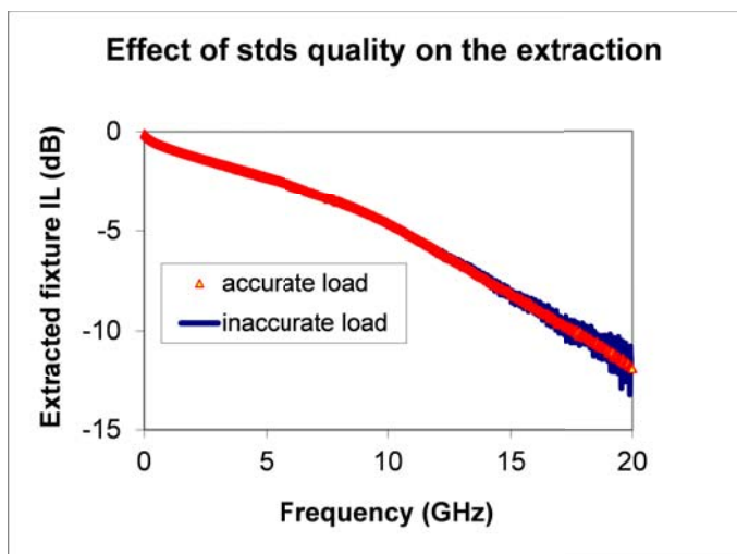
Figure 8-17. The effect of a load standard problem on extracted insertion loss with type B. Eventually, the load accuracy does matter.
