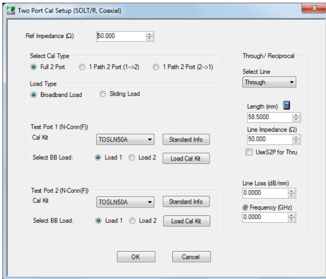
Figure 3-1. TWO PORT CAL SETUP (SOLT/R, COAXIAL) Dialog Box
