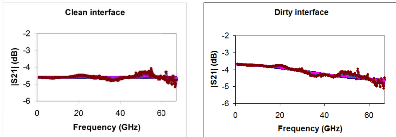
Figure 8-19. The sensitivities of a type D extraction to underlying calibration issues (multiple traces per plot, reflect magnitude variations) and introduction of an inner plane match and position problem (the dirty interface plot).
