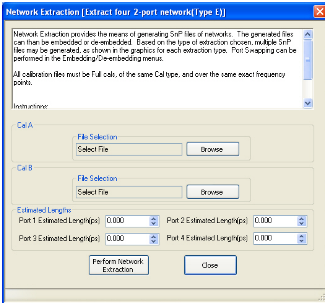
Figure 16-31.NETWORK EXTRACTION TYPE E Dialog Box
