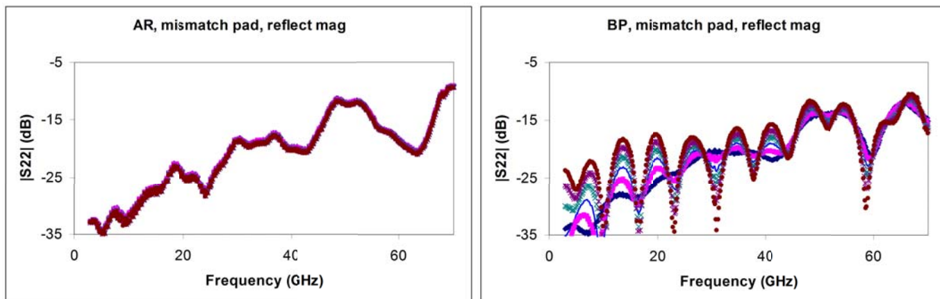
Figure 8-16. A comparison of output match sensitivity for type A (AR) and type B (BP) methods.
