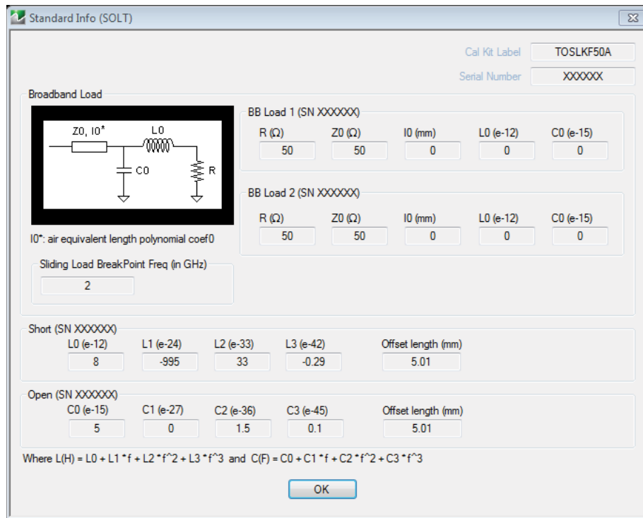
Figure 3-5. STANDARD INFO (SOLT/R)
