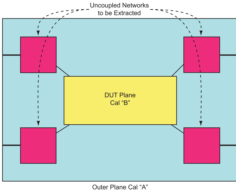
Figure 16-32. Type E Network Extraction - Uncoupled Networks To Be Extracted
