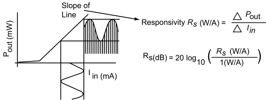
Figure 18-2. The concept of responsivity is shown here. The conversion parameters of the O/E and E/O devices measured with the VNA are essentially measures of responsivity.
