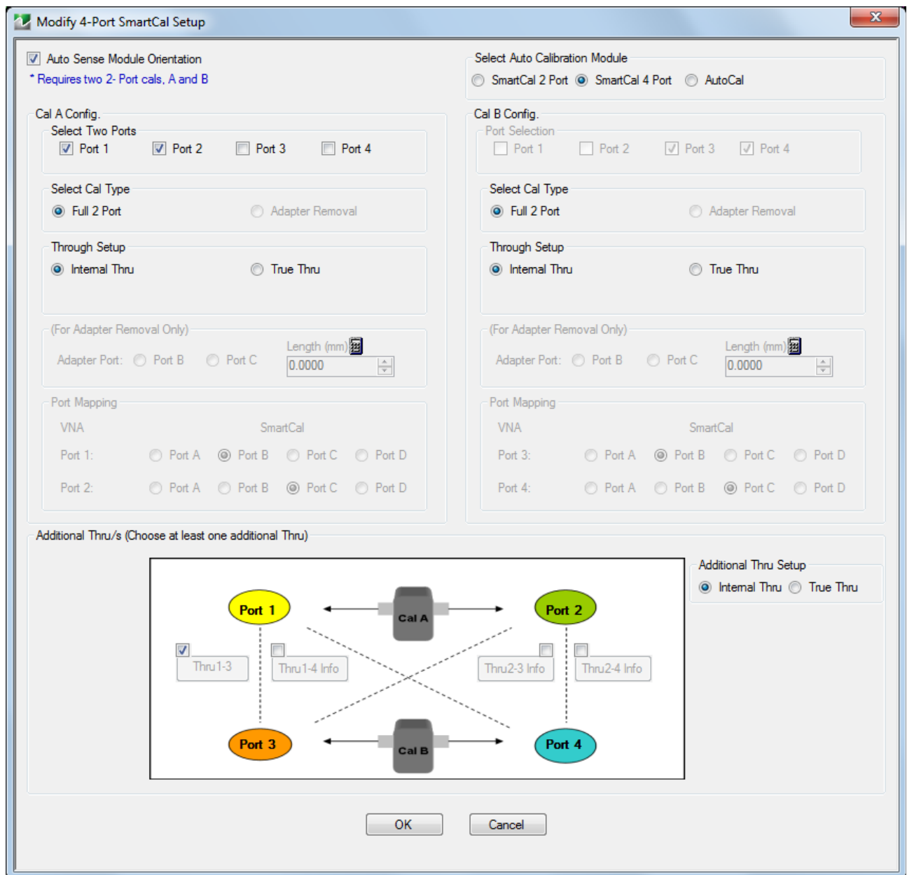
Figure 2-18. MODIFY 4-PORT SMARTCAL SETUP DIALOG – SmartCal 4-Port Selected
