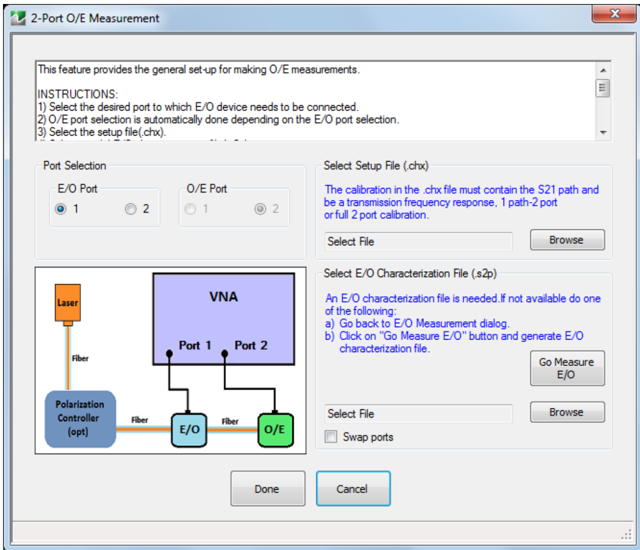
Figure 18-8. The dialog for 2-port O/E measurements is shown here.
