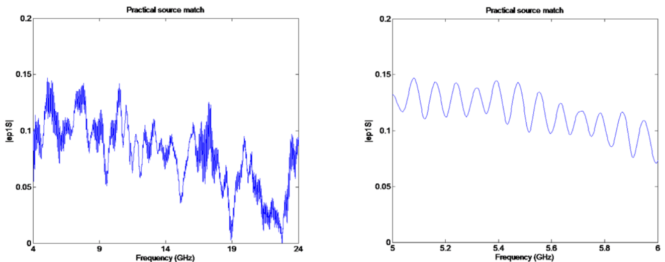
Figure 9-5. Large scale and zoomed-in source match variation over frequency.
