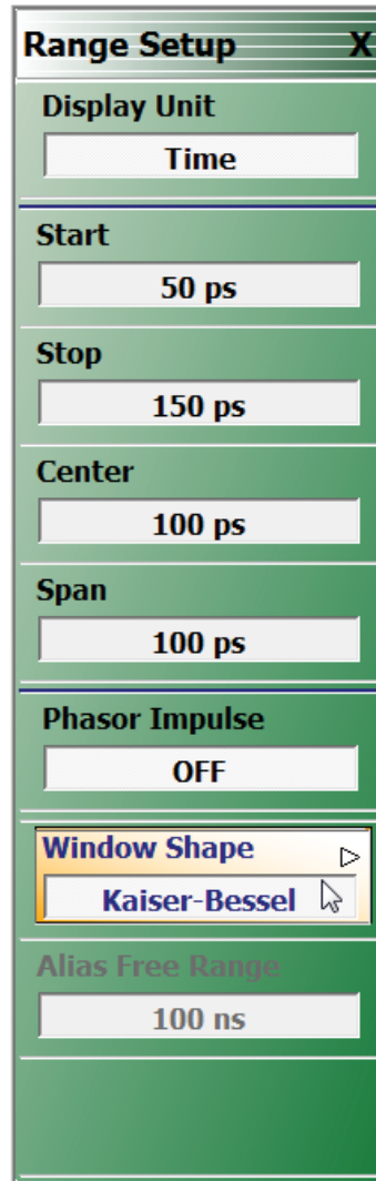
Figure 12-13. RANGE SETUP Menu for Bandpass Time Domain
