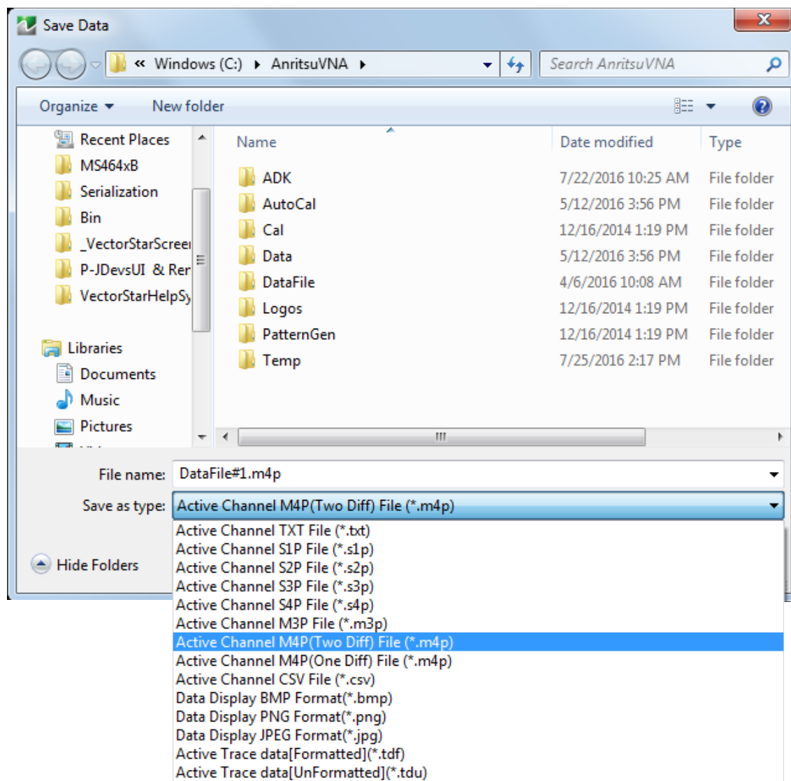
Figure 16-27. The file save options are shown here to include the .mNp format. Note that there are two choices for .m4p depending on if the setup is for two differential pairs or one differential pair (and two singletons).
