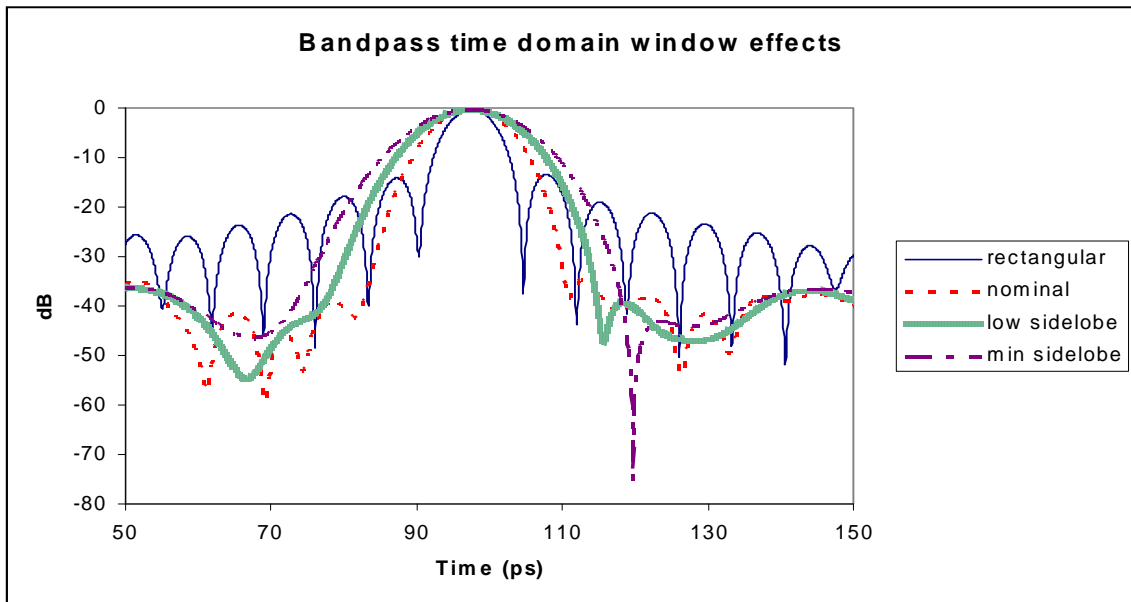
Figure 12-14. Window Effects in Bandpass Time Domain
