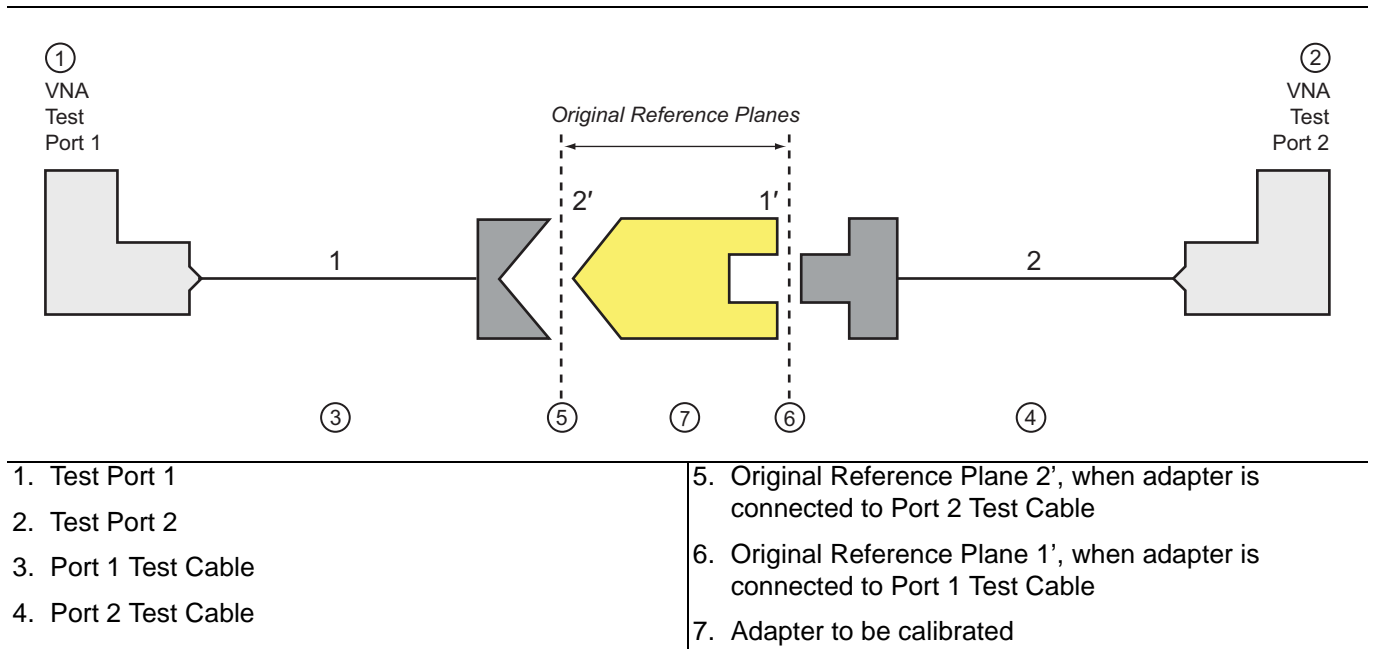
Figure 8-7. Adapter Removal Block Diagram
