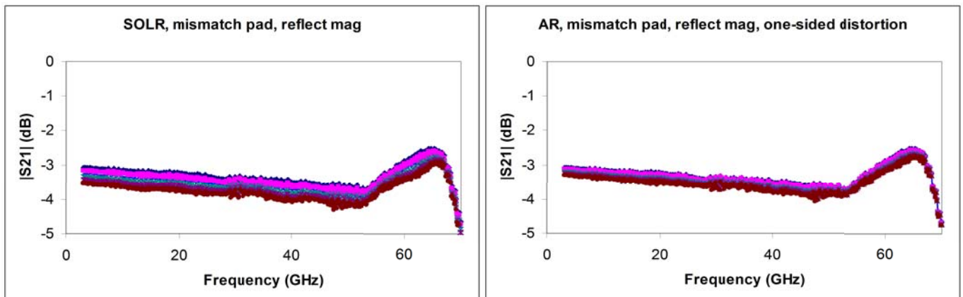
Figure 8-15. A comparison of the effects of a reflect standard problem on both a type A extraction (AR) and a SOLR calibration.
