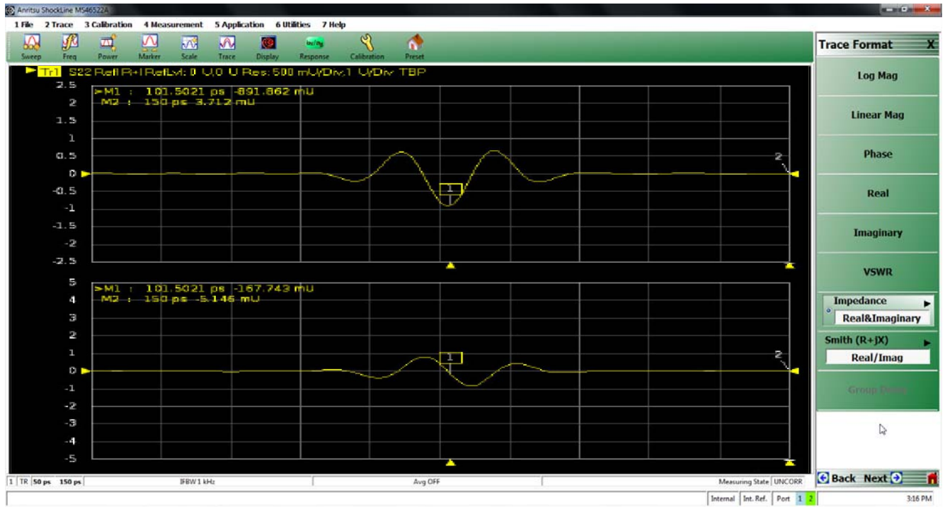
Figure 12-12. Example Band-pass Time Domain Plot
