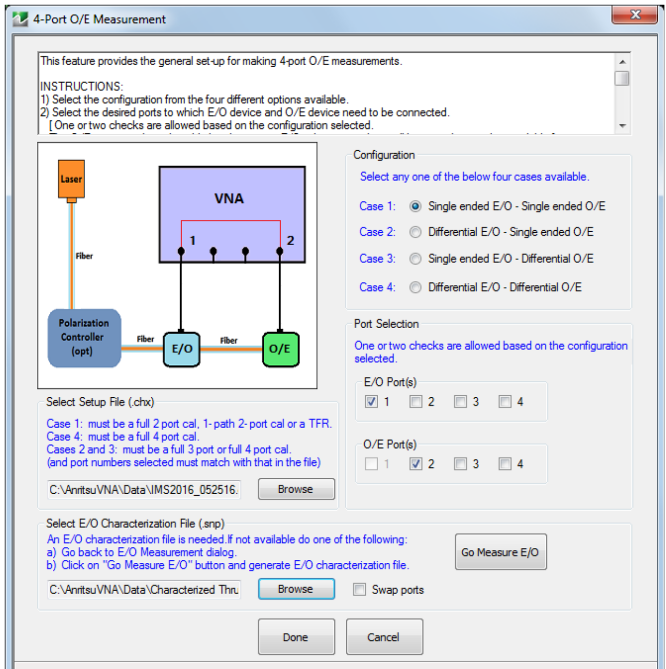
Figure 18-13. The dialog for 4-port O/E measurements is shown here.
