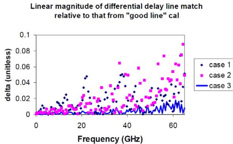
Figure 16-24. Measurement Uncertainties for Through and Reciprocal Selection
