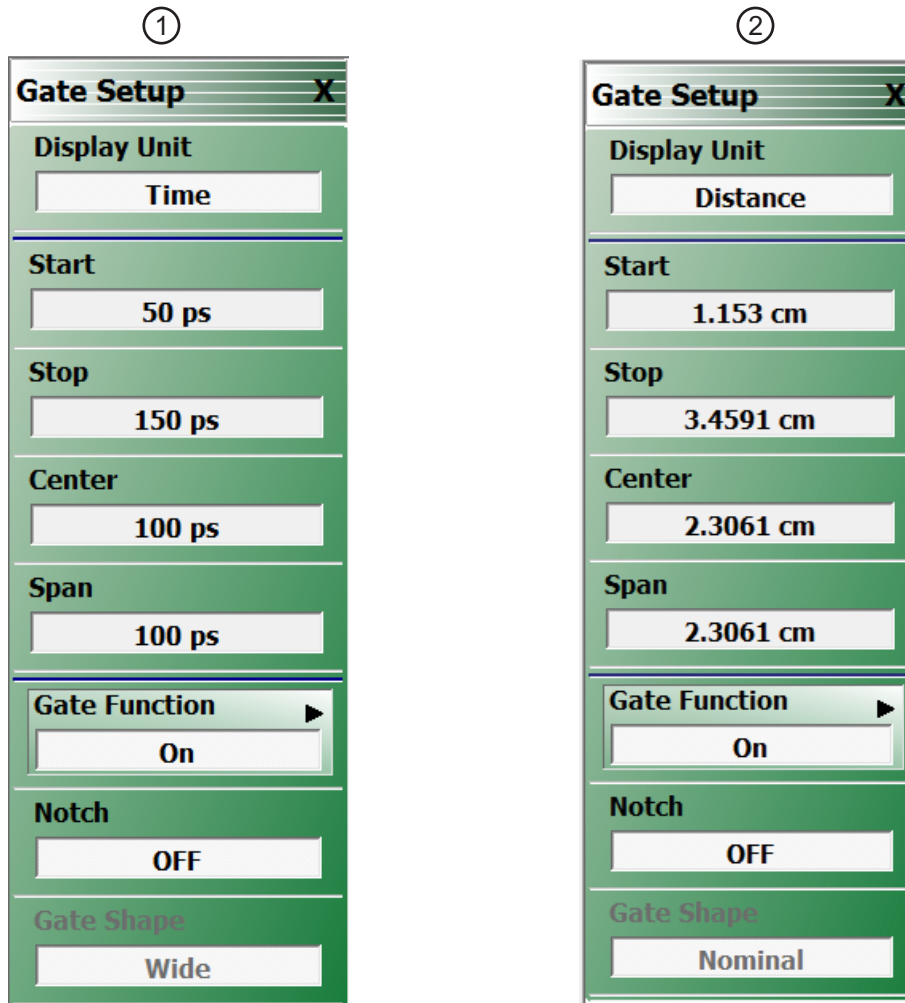
Figure 12-16. GATE SETUP Menu
