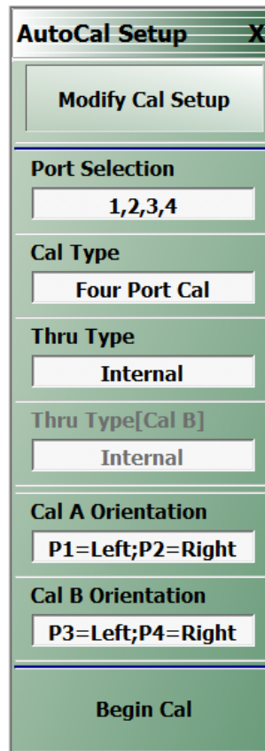
Figure 2-21. Configured SmartCal 2-Port Menu Setup
