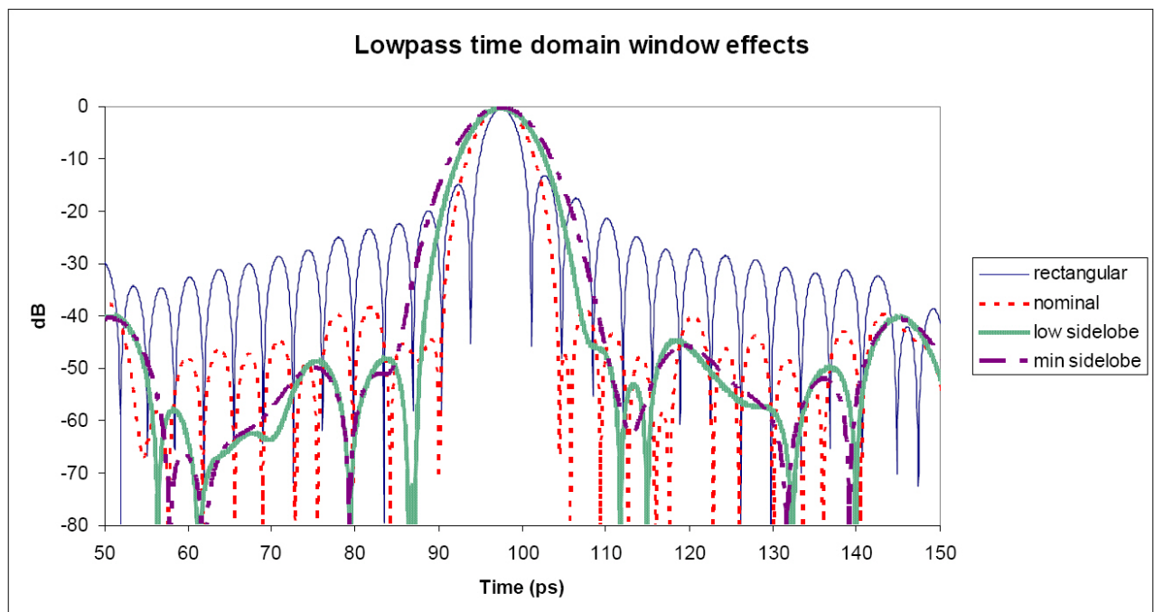
Figure 12-7. Effects of Window Shapes Plot
