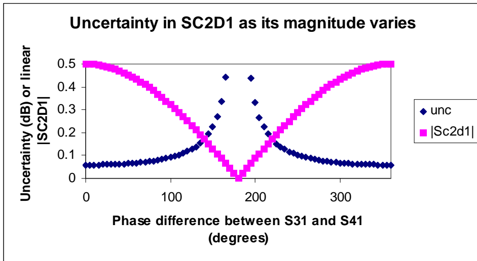
Figure 16-25. SC2D1 Uncertainty in SC2D1
