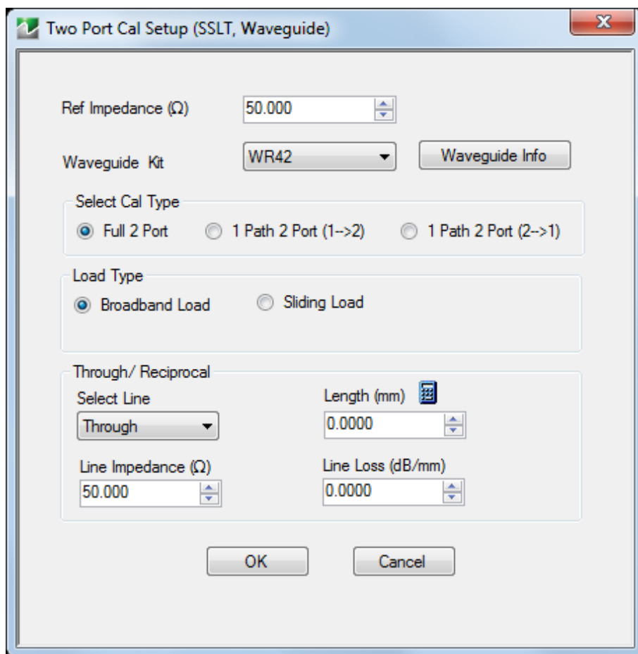
Figure 4-2. TWO PORT CAL SETUP (SSLT, WAVEGUIDE) Dialog Box
