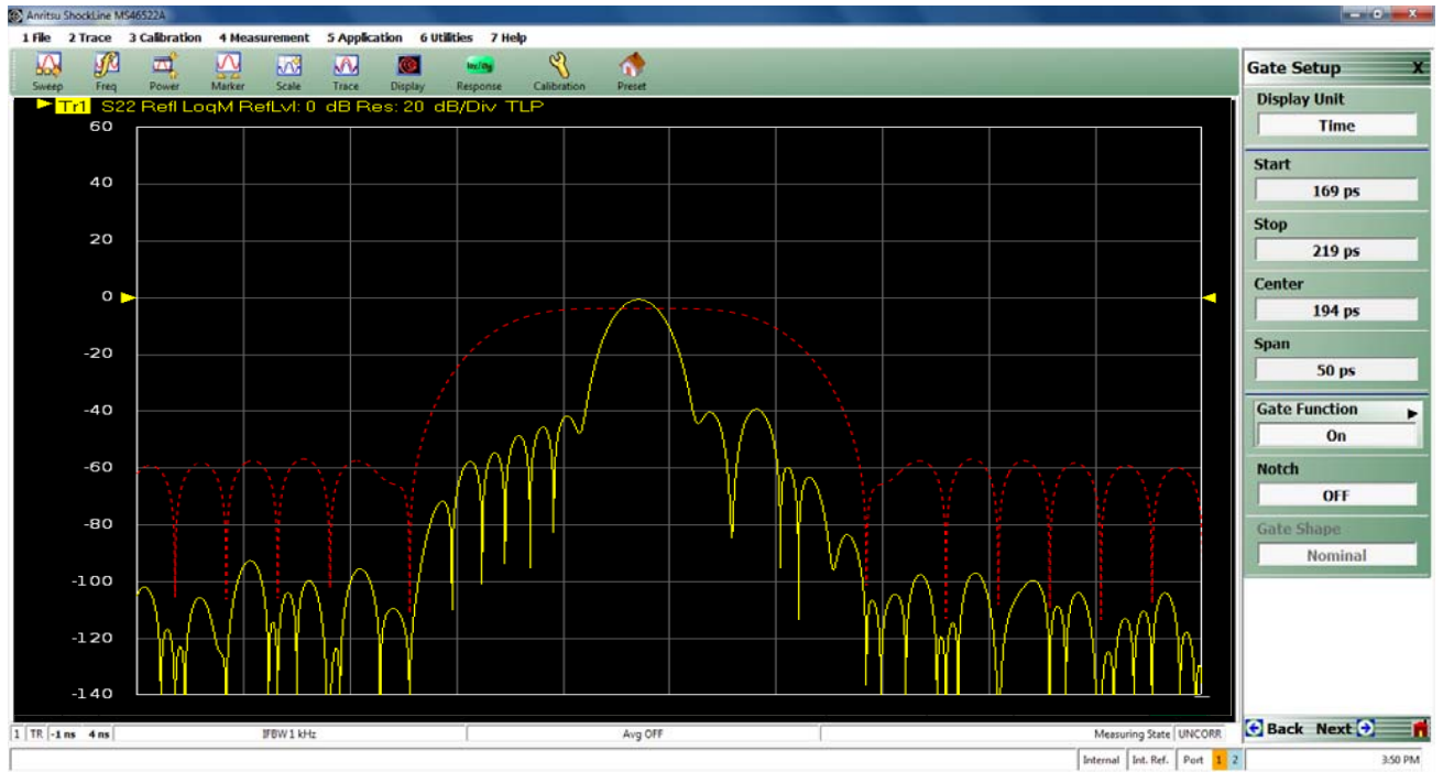
Figure 12-19. Gate Turned On Example
