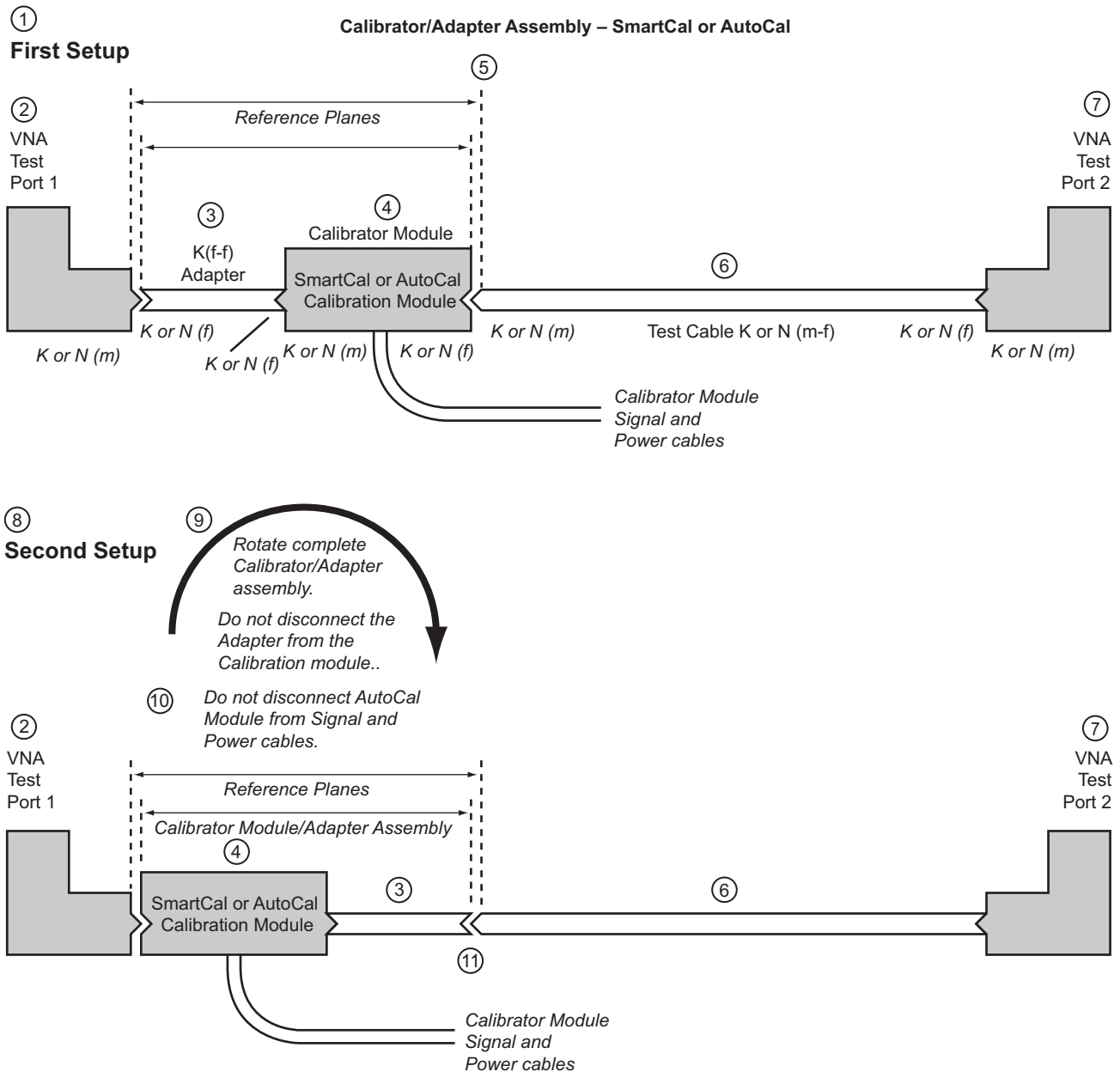
Figure 2-29. Calibrator, Adapter Removal, Internal Thru (1 of 2)
