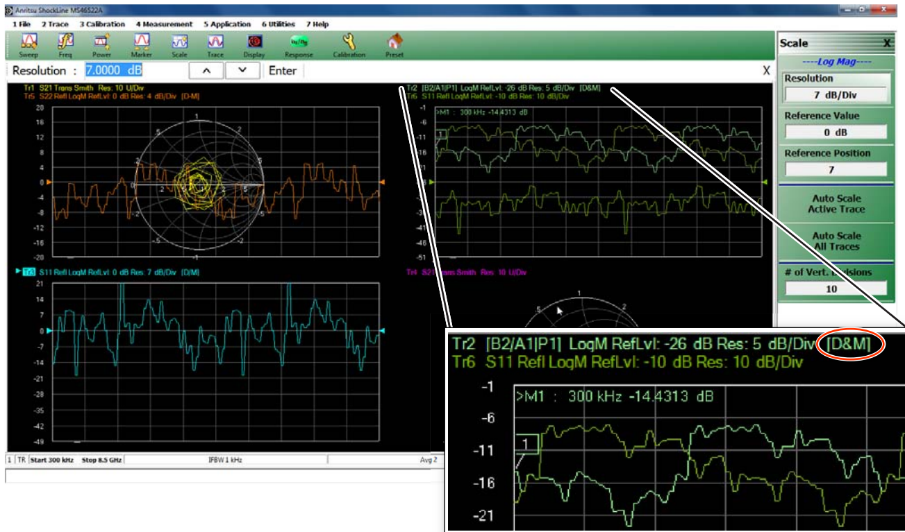
Figure 11-9. Multi-Trace Display with right-side SCALE menu
