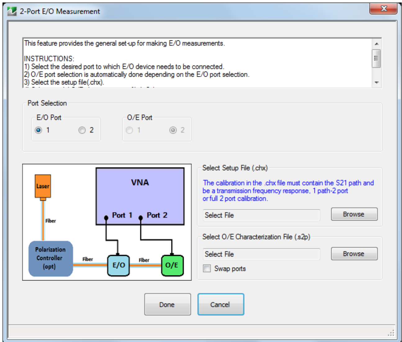
Figure 18-7. The dialog for 2-port E/O measurements is shown here.
