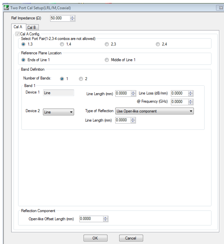
Figure 6-7. Calibration Setup Dialog - TWO PORT CAL SETUP (LRL/LRM, COAXIAL) Dialog Box
