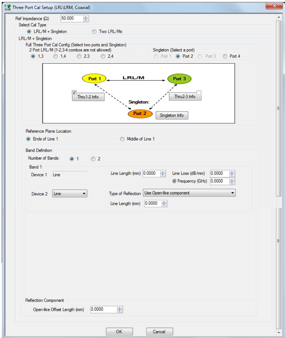
Figure 16-19. THREE PORT CAL SETUP (LRL/LRM, COAXIAL) Dialog Box - LRL/M + Singleton
