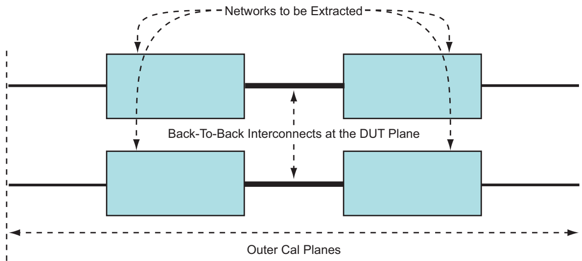
Figure 16-34. Type F Network Extraction - Back-to-Back Interconnects at the DUT Plane - Type F
