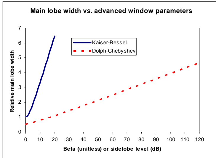
Figure 12-10. Comparison of Lobe Width vs. Window Parameters
