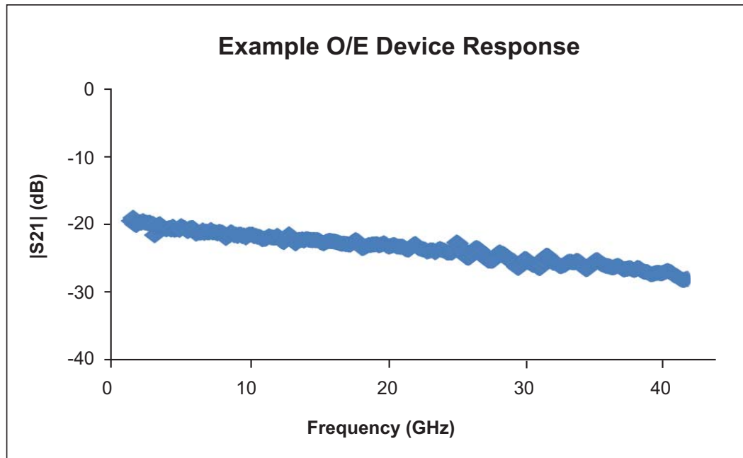
Figure 18-4. The characteristics of an example O/E device are shown here. (2 of 2)
