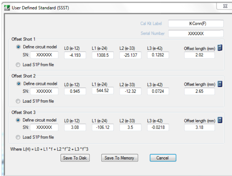
Typical parameters for SSST calibration - K (F) Connectors
