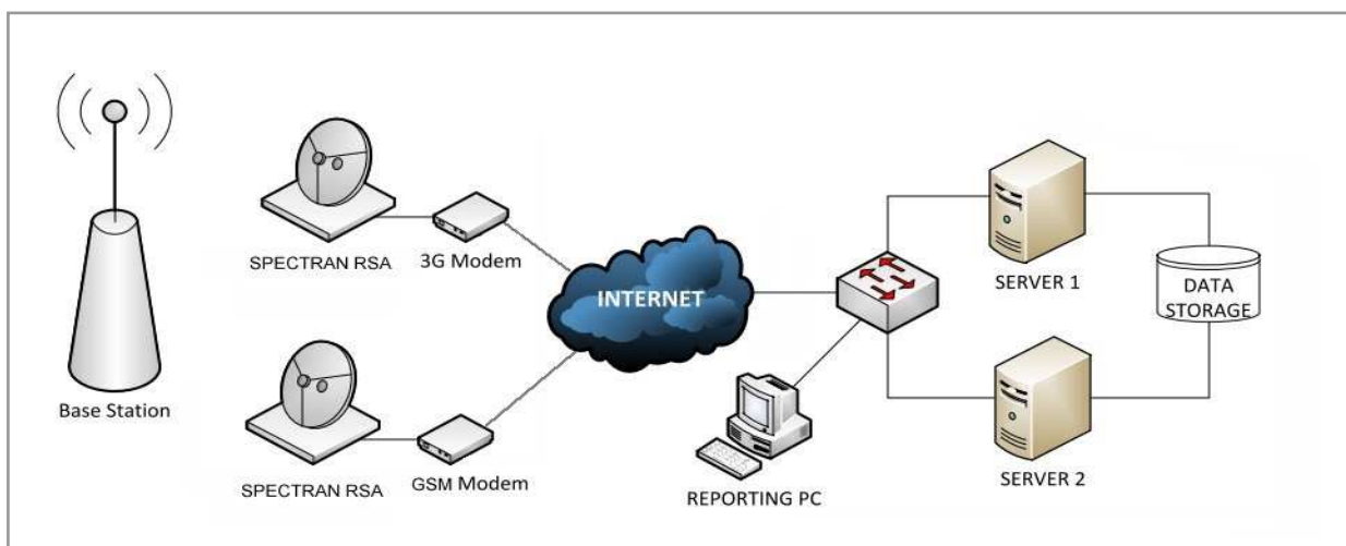
Example of a typical measurement setup using multiple SPECTRAN RSA units with „EMF-Monitor“ Software installed, all captured measurement data are continuously stored on the SPECTRAN RSA or Webservice and can be accessed through any PC
