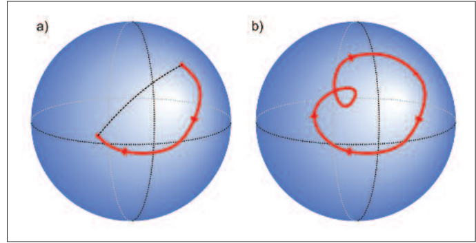
Figure 17. SOP can be conveniently represented in the so-called Poincaré Sphere. PDM receivers must keep track of the instantaneous SOP which evolves rather slowly over time. AWGs can produce any trajectory of the SOP over the Poincaré Sphere in order to stress receivers. However, to be useful, record length must be extremely long to reproduce speeds and frequencies within the range of the receiver-under-test' SOP tracking system. For continuous signal generation, which requires looping the same waveform, open trajectories like the one shown in (a) are not acceptable as the instantaneous discontinuity will confuse the receiver. SOP trajectories must be closed, like the one in (b), for continuous, seamless signal generation.
