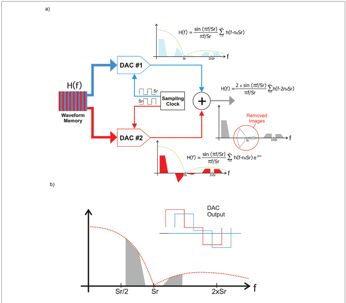
Figure 6. Interleaving-DAC AWGs can double the effective sampling rate as the two channels convert alternative samples delayed by half the sampling period (a). In this way, images located in the second Nyquist band (from Sr/2 to Sr ) are nulled and any signal from DC up to Sr may be implemented.
