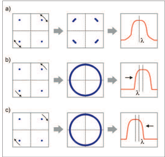
Figure 15. Laser linewidth can be also emulated electrically by rotating the constellation back and forth resulting in phase noise (a). Clock-wise (c) or counter-clockwise (b) constant speed rotation of the constellation can be used to shift the \lambda of the optical carrier in either direction.
