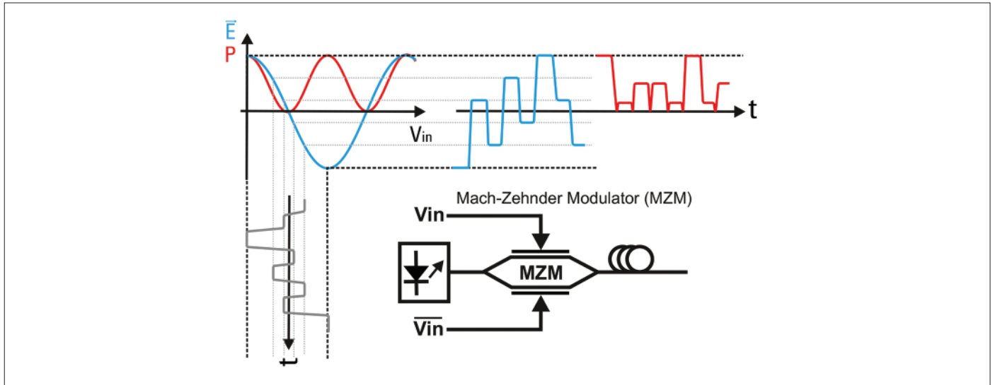
Figure 3. Mach-Zehnder Modulators are non-linear devices and require relatively high amplitude voltage swings to work. They may be driven by single-ended or differential electrical signals. Linearity is an important requirement for proper multi-level modulation. Here a 4-level electrical signal (one of the baseband components of a QAM16 signal) is distorted so electrical field at the output of the modulator remains linear.
