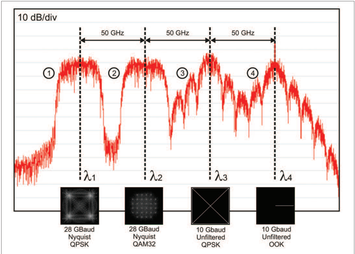
Figure 1. Spectral efficiency of optical transmissions may be improved by modulating both the amplitude and the phase of an optical carrier, which requires coherent modulation and detection. In this WDM link, four different wavelengths share the same fiber in a standard ITU 50GHz grid. Wavelength 4 is carrying a 10Gb/s signal using the traditional intensity modulation (or On-Off Keying, OOK). Part of the optical power goes directly to the carrier and does not transport any information. Carrier 3 is modulated using a QPSK modulation so 2 bits are transported by each symbol, doubling the capacity of the OOK-modulated channel in the same bandwidth. Capacity may be increased through the usage of more complex modulations or baseband filtering. Wavelengths 1 and 2 transport 28 Gbaud signals with 2 and 5 bits per symbol respectively.
