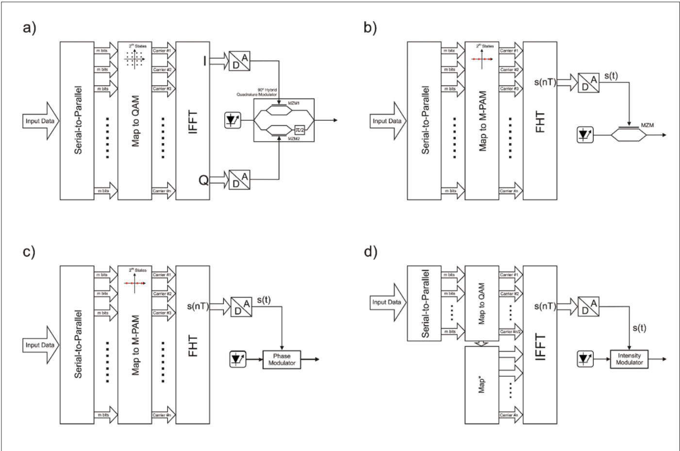
Figure 4. OFDM (Orthogonal Frequency Division Multiplex) signals are extremely popular in the wireless world. Their resilience to linear distortions introduced by the network such as Chromatic Dispersion (CD), or Polarization Mode Dispersion (PMD), and their inherent limited bandwidth make them very attractive for optical transmission as well. OOFDM (Optical-OFDM) is based in different modes other than the traditional Complex-FFT approach so popular in wireless and broadcast networks (a). Some less efficient schemes are being experimented in exchange for simplicity or cost. Some are based in the Fast Hartley Transform (FHT) (b, c) which result in a real-only signal so quadrature modulator is not necessary. In some cases, it is even possible to avoid the usage of coherent optics by using direct modulation (d). Peak-to-average-power ratio0 is an important drawback of OFDM signals. In c) the same real-only OFDM signal is modulating the phase of an optical carrier, not the amplitude, so optical power does not change over time.
