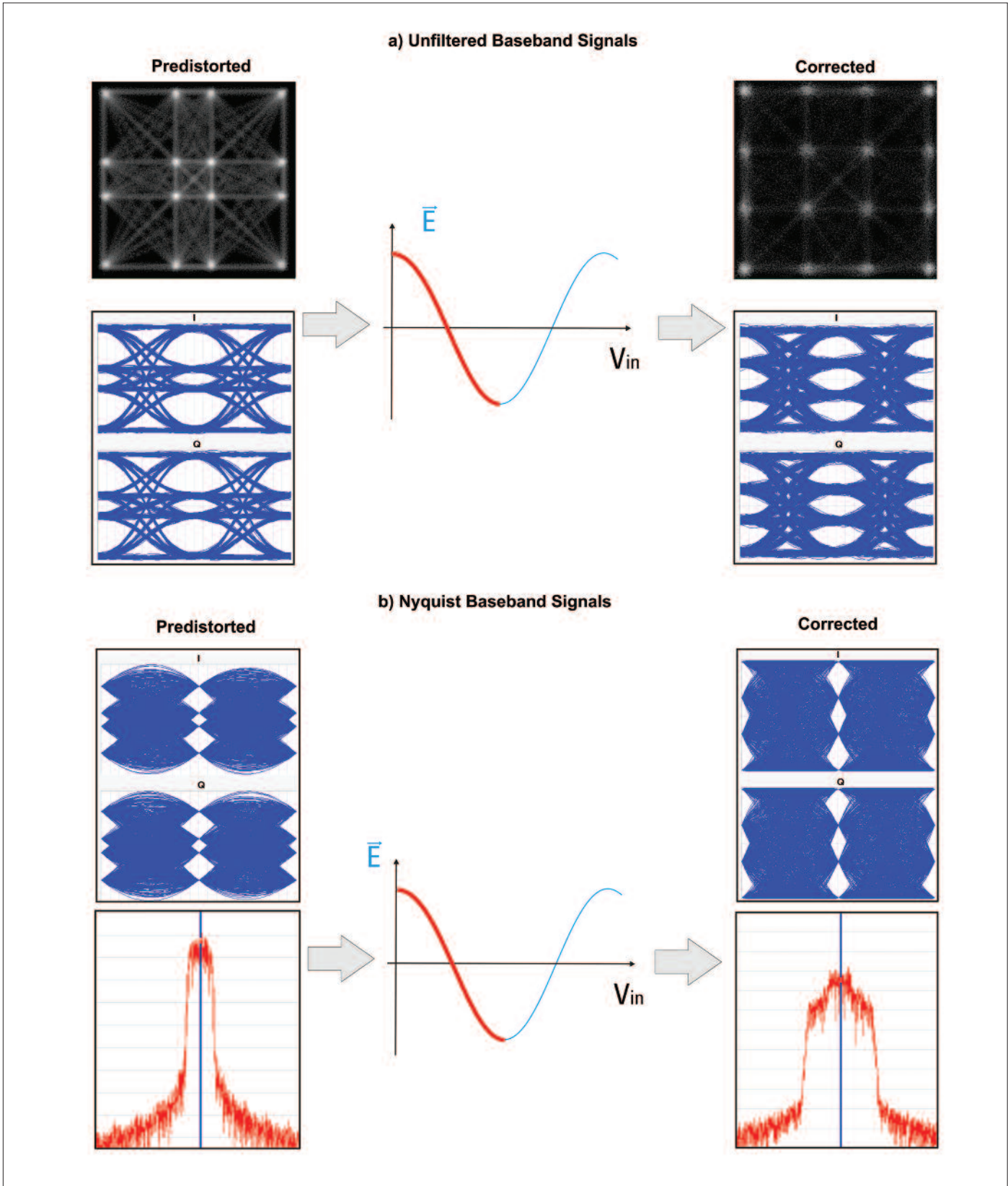
Figure 11. Non-linear behavior of MZM is an important issue for complex modulation. For unfiltered, fast baseband signals it is enough to pre-distort the electrical levels to obtain perfect signals (a). For bandwidth limited signals, such the ones used in Nyquist or quasi-Nyquist channels, this is not enough as non-linear distortion results in spectral growth and a increased bandwidth so adjacent channels may be interfered (b).
