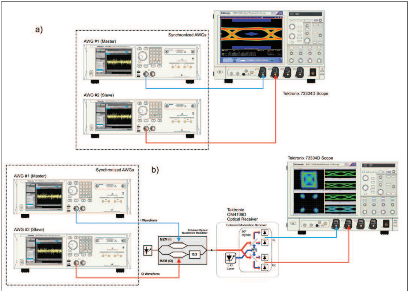
Figure 14. Joint channel, or even instrument, calibration and correction are important to obtain the best results. Electrical-only calibration (a) is a straight-forward operation if the right measurement devices, such as the Tektronix DPO/DSA70000 oscilloscopes, series are available. Complete system (including the optical components) calibration and characterization require a Optical Modulation Analyzer (b) such as the Tektronix OM4106D.
