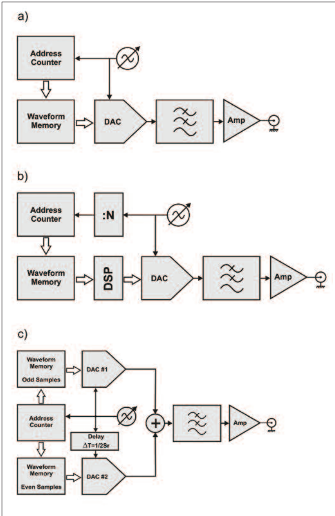
Figure 5a, b, c. Arbitrary Waveform Generator block diagram look close to that of a digital storage oscilloscope, or DSO (a). “True-arb” architectures (a) transfer samples from a waveform memory to the DAC at its conversion speed. Interpolating-DAC AWGs (b), transfer samples from the memory at a fraction of the DAC’s sampling rate so intermediate samples must be interpolated. Although this architecture has some advantages, actual signal bandwidth is primarily limited by the memory transfer speed. DAC-interleaving AWGs, such as the Tektronix AWG7000 and AWG70000 series, can combine two AWG channel to effectively double the sample rate of the instrument so sampling rates as high as 50GSa/s may be reached.
