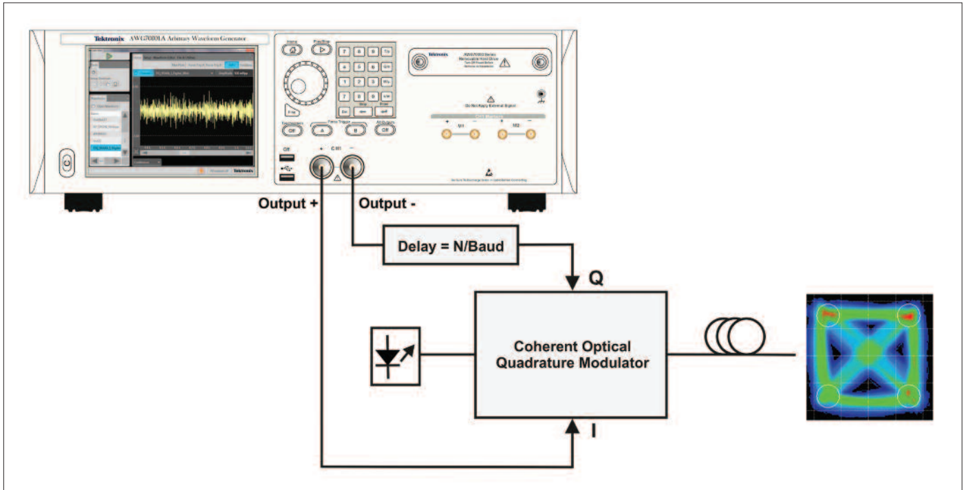
Figure 18. Some modulation schemes may be generated by single channel instruments. Uncorrelated I and Q baseband signals may be obtained by delaying one of them by an integer number of symbol times. Here, the two complementary outputs of a Tektronix AWG70000 series generator are used in such an arrangement, providing for higher amplitude signals than those coming out from a power splitter fed by one of the outputs.
