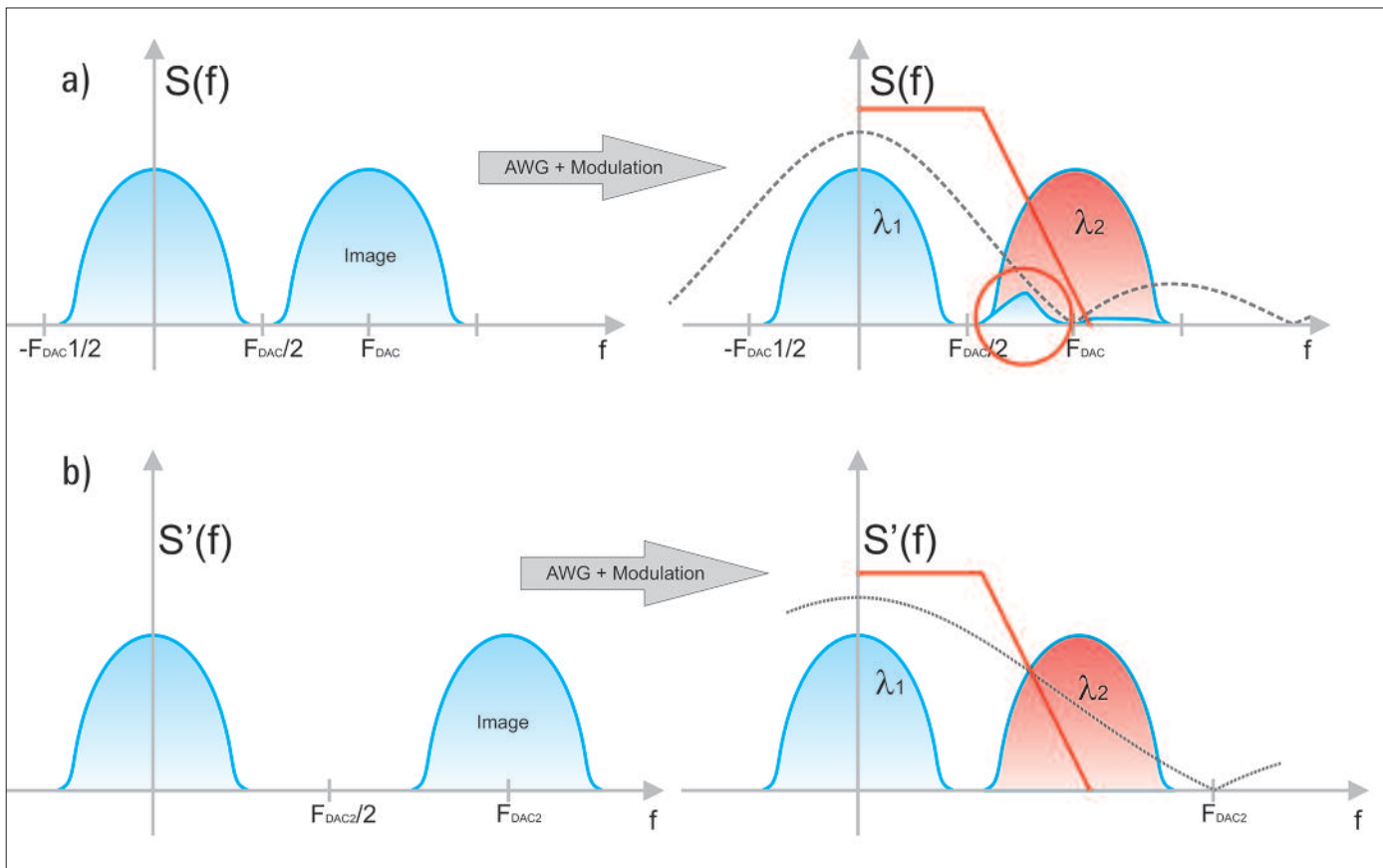
Figure 12. The higher the AWG sampling rate the better, even if it is larger than the required for a given signal according to the sampling theorem (2B). Increasing sample rate results in a flatter frequency response and a larger distance to the first unwanted image. In (a), the DAC sampling rate is enough for the signal, but insufficient filtering result in an image interfering the adjacent optical channel (in red). The same filter produces no interference in a higher sampling rate AWG (b) as the image is completely removed from the modulator's output.
