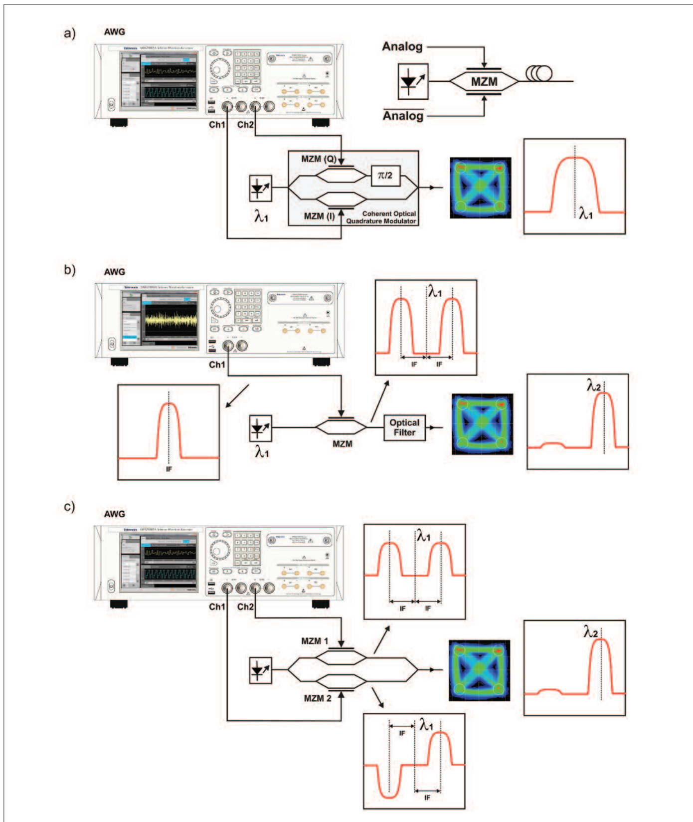
Figure 10. There are several ways to obtain complex modulated signals in the optical domain other than a two-channel arb and a quadrature modulator (a). Fast enough one-channel AWGs can generate a IF signal that can be up-converted through an amplitude modulator (b). The output will consist of two modulated carriers so one of them must be removed through filtering. A two-channel generator can generate two almost identical IF signals with the exception of the phase for each carrier and applied to two balanced amplitude modulators to get rid of one of the images. Notice that the phase of the optical carrier is the same for both modulators.
