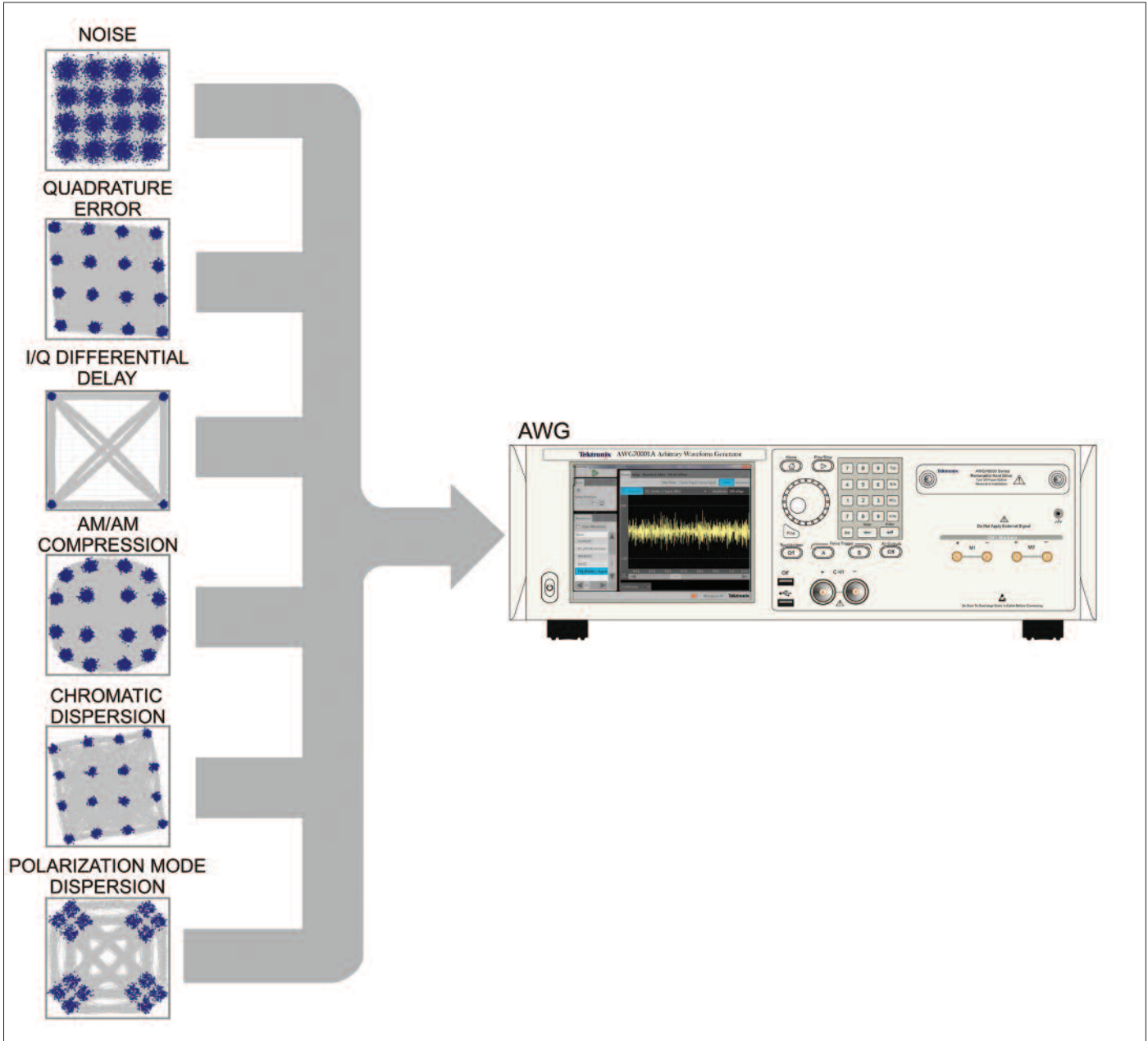
Figure 13. AWGs can produce a large variety of distortions, linear and non-linear, applied to modulated signals. These can emulate issues in the transmitter, the receiver, and even the link or the network. The same capability can be used to compensate for such distortions and obtain better-quality signals from poor-quality components or links.
