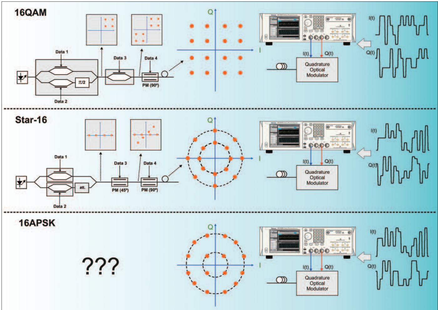
Figure 9. Some complex modulations can be generated by directly applying two-level signals (i.e from a high-speed pattern generator) to optical modulation components. For some modulation schemes, though, this is difficult or even impossible. Here, a square-constellation QAM16 and a STAR16 modulation schemes are implementing using this approach. However, a 16APSK constellation cannot be implemented in this way. Notice the difference in the modulators components and their connection. All these modulation schemes can be generated through the combination of a two-channel AWG and an optical quadrature modulator. Additionally, AWGs can be set-up to generate distorted signals without any change in the hardware.
