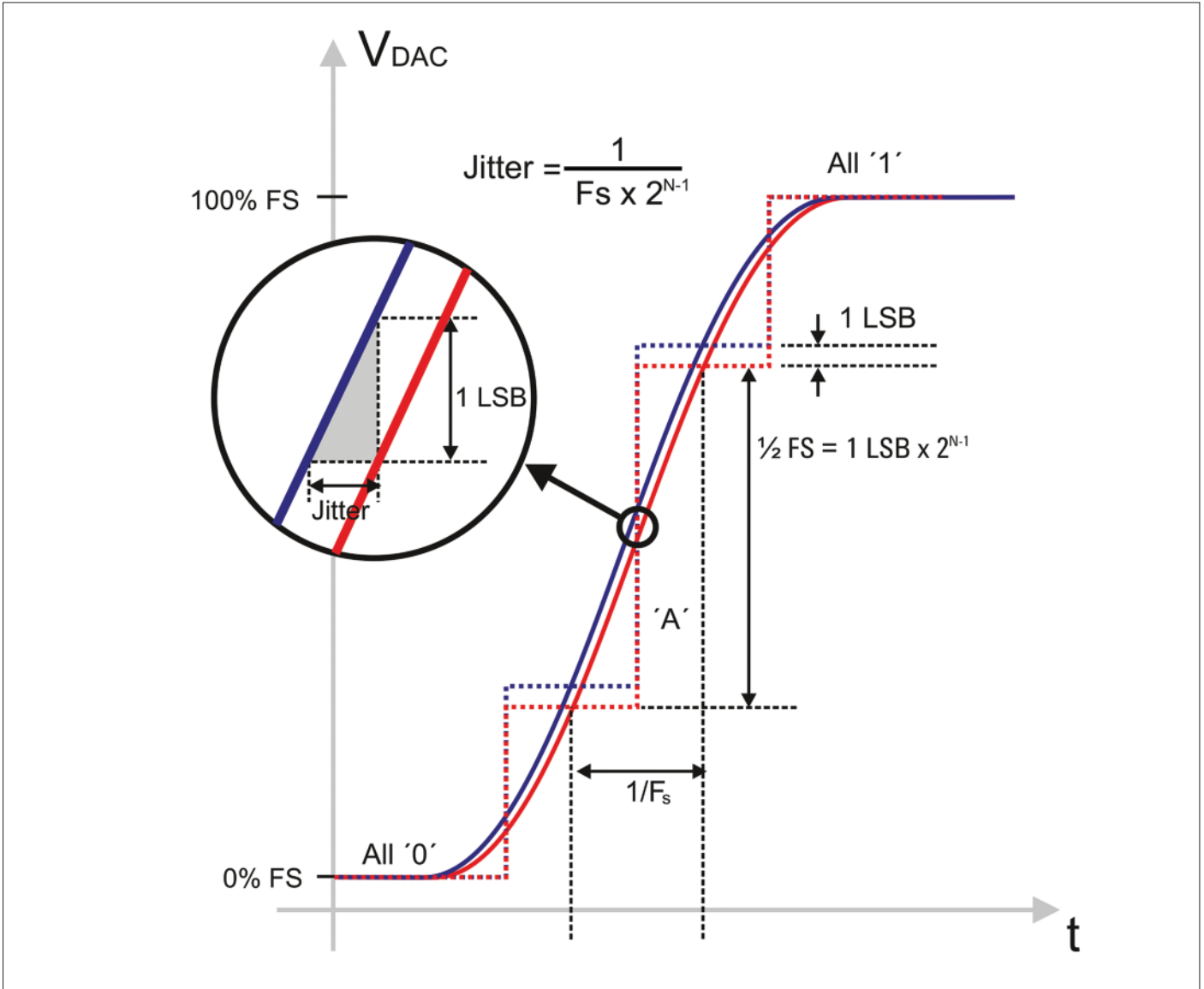
Figure 8. The edge positioning capability of any AWG depends on two main factors: sampling rate and vertical resolution. Edge positioning granularity translates into increased intrinsic jitter. In a 6-bit vertical resolution AWG, this component of jitter will be 16 times larger than that of a 10-bit vertical resolution AWG, such as the Tektronix 70000 series.
