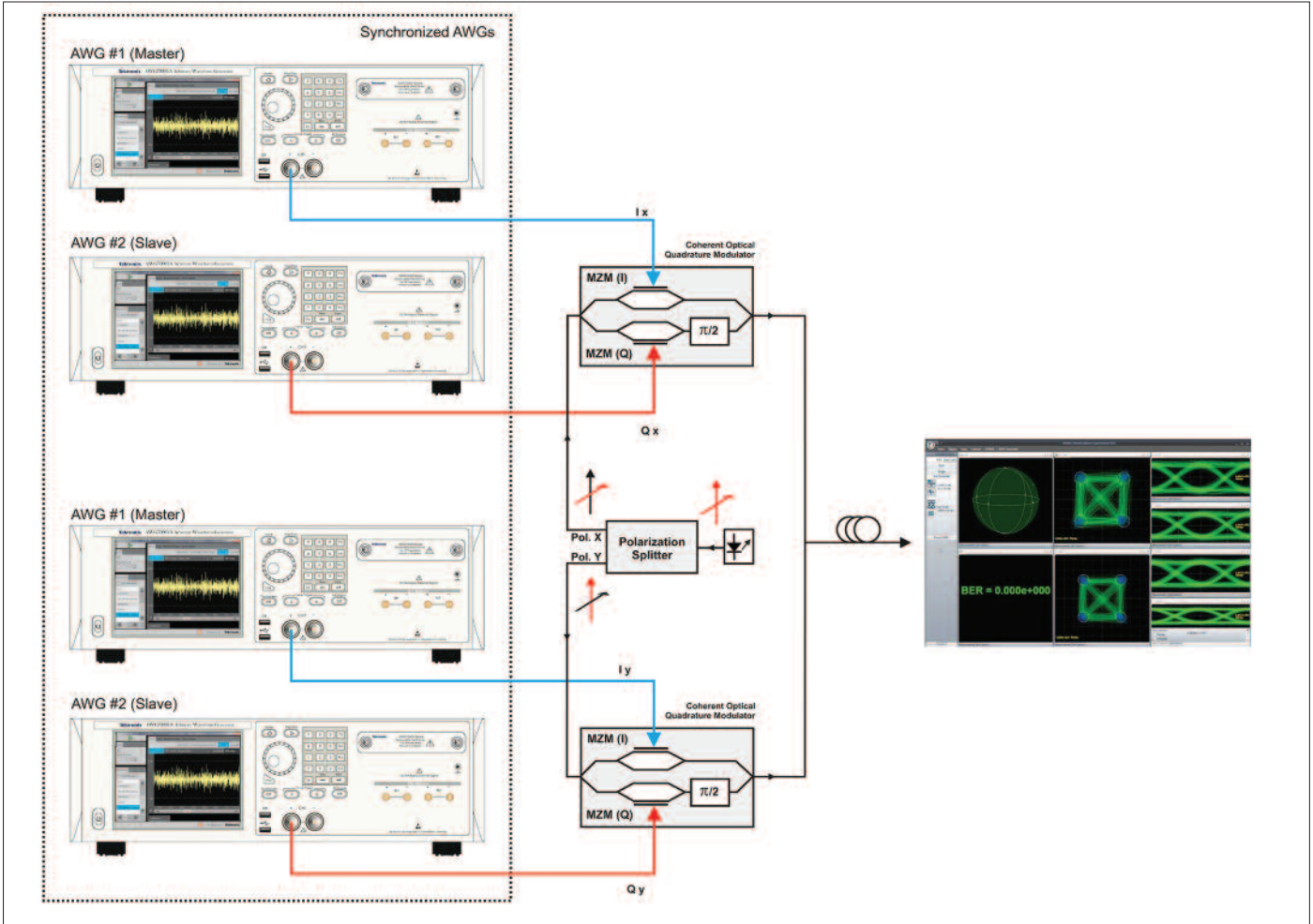
Figure 16. Complete Polarization Division Multiplexed transmitter emulation requires 4 synchronized AWG channels to generate the I_x , Q_x , I_y , and Q_y baseband signals. Adequate control of those 4 signals can be used to emulate any static or dynamic SOP (State-Of-Polarization).
