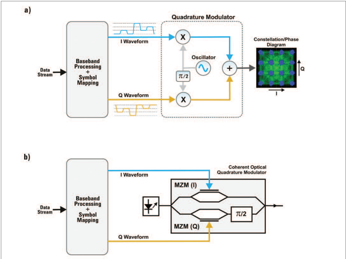
Figure 2. One way to modulate the amplitude and the phase of a carrier is a quadrature modulator. There, two baseband signals, called I (or In-phase) or Q (Quadrature), modulate in amplitude two orthogonal carriers (90° relative phase) so any state of modulation can be accomplished. The same scheme may be implemented for optical carriers by using two Mach-Zehnder Modulators (MZM) in an arrangement known as “Super-MZM” cell.
