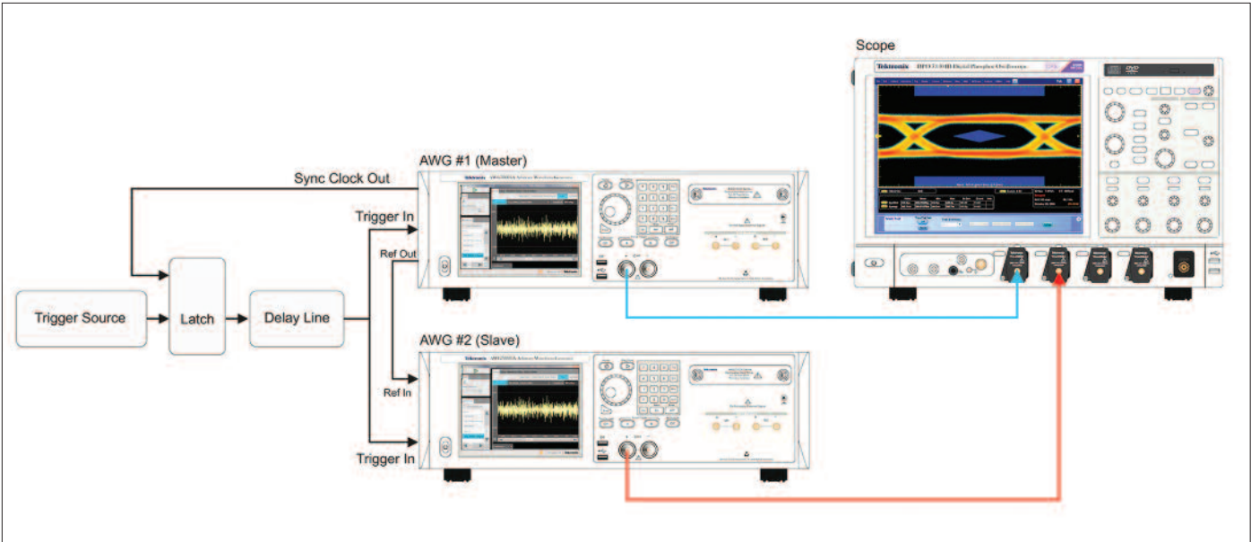
Figure 7. Complex modulation requires multiple synchronous baseband signals (up to 4 in a Polarization Division Multiplex link). Synchronizing multiple AWGs is extremely important to obtain useful signals. Here, the recommended multi-instrument synchronization scheme for the Tektronix AWG70000 series is shown. With this arrangement, channel-to-channel skews better than 4ps can be obtained.
