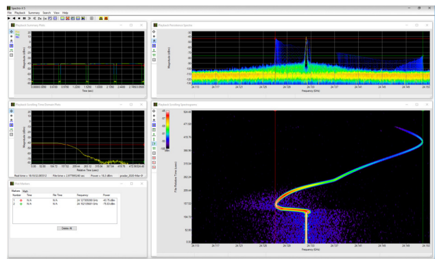
IQ file compatibility with Bird Spectro-X software for post-processing can highlight detailed information on a radar pulse pre- and post-signal drift with \mu s resolution
