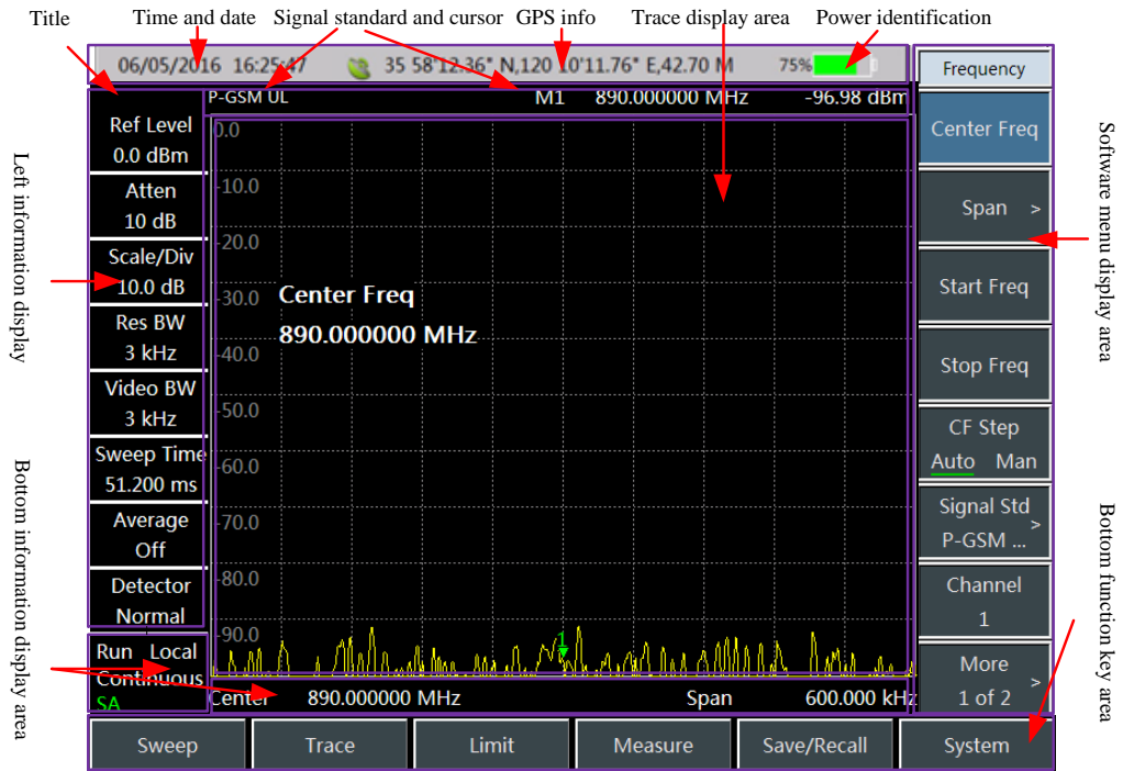
Fig. 2.2 Operation interface of 4024 Spectrum Analyzer
