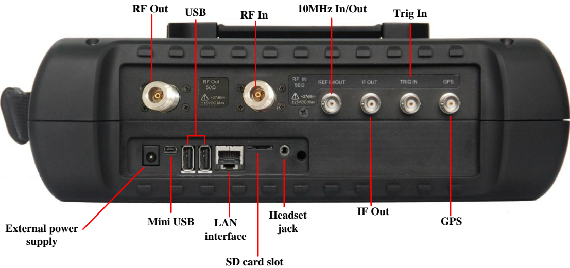
Fig. 2.3 Top panel of 4024 Spectrum Analyzer
