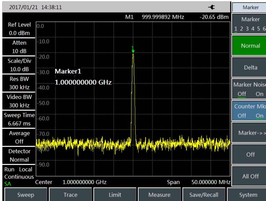
Fig. 3.6 Use marker function to improve frequency measurement accuracy
