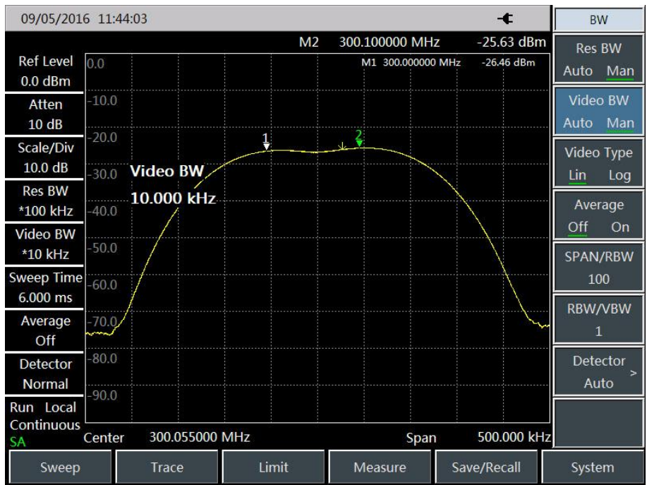
Fig. 3.13 Able to distinguish two signals of same amplitude
