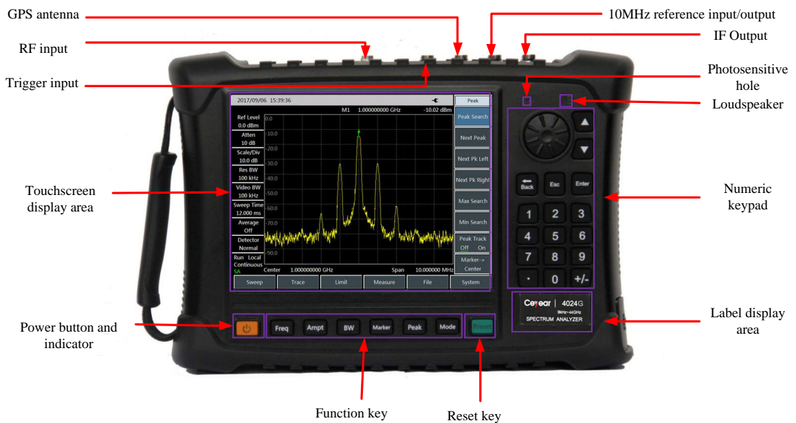
Fig. 2.1 Front panel of 4024 Spectrum Analyzer
