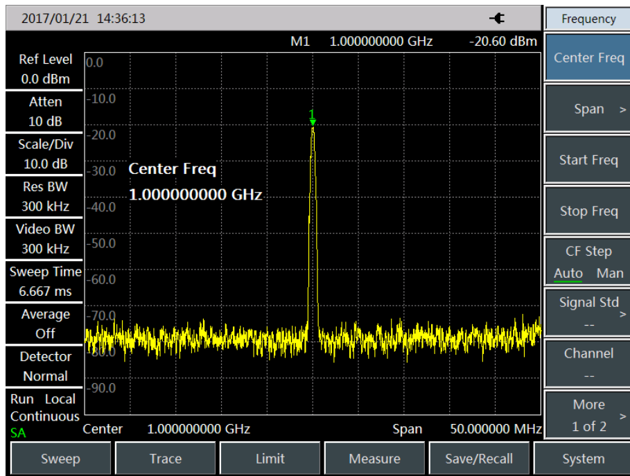
Fig. 3.1 Center frequency is 1GHz
