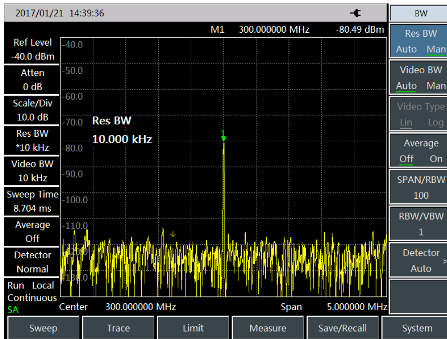
Fig. 3.9 Reduce resolution bandwidth to measure small signals
