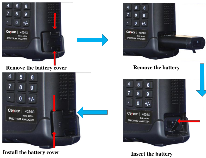
Fig. 2.4 Install or replace the battery
