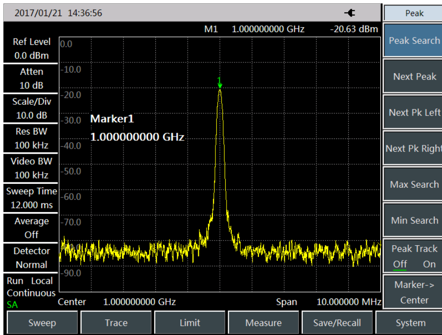
Fig. 3.3 Activate the marker
