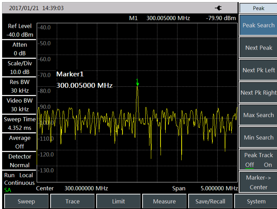
Fig.3.7 Small signal when pre-amplifier Off
