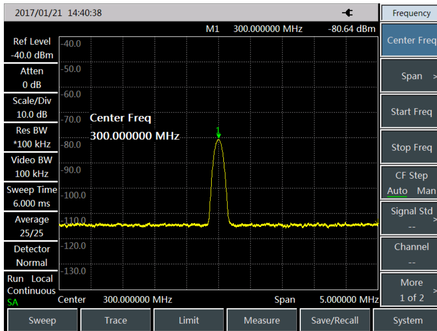
Fig. 3.10 Measure small signals with trace average
