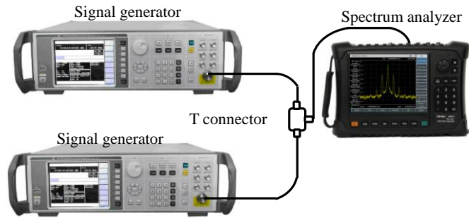
Fig. 3.11 Test instrument connection diagram of two input signals
