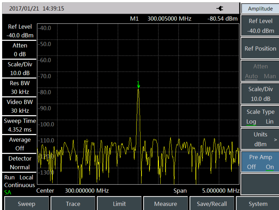
Fig. 3.8 Small signal when pre-amplifier On
