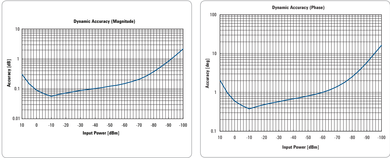
Figure 17. Dynamic Accuracy Option 3L5
