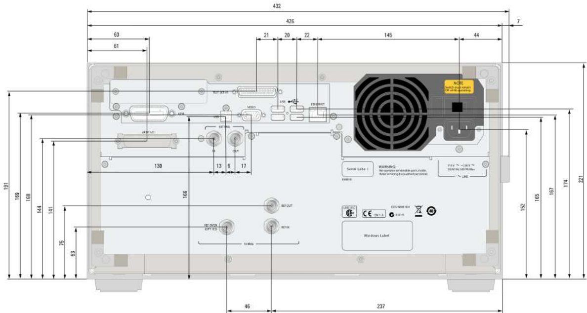
Figure 22. Dimensions (rear view, in millimeters)
