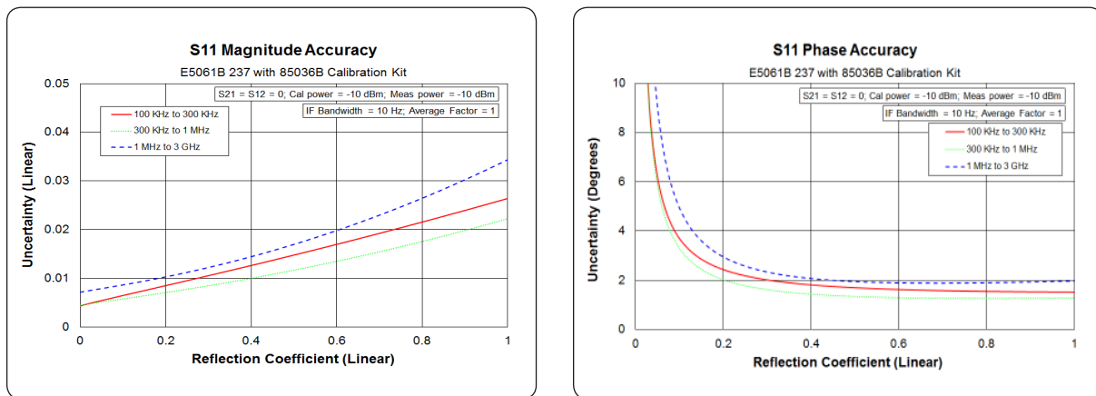
Figure 16. Reflection uncertainty (specification)
