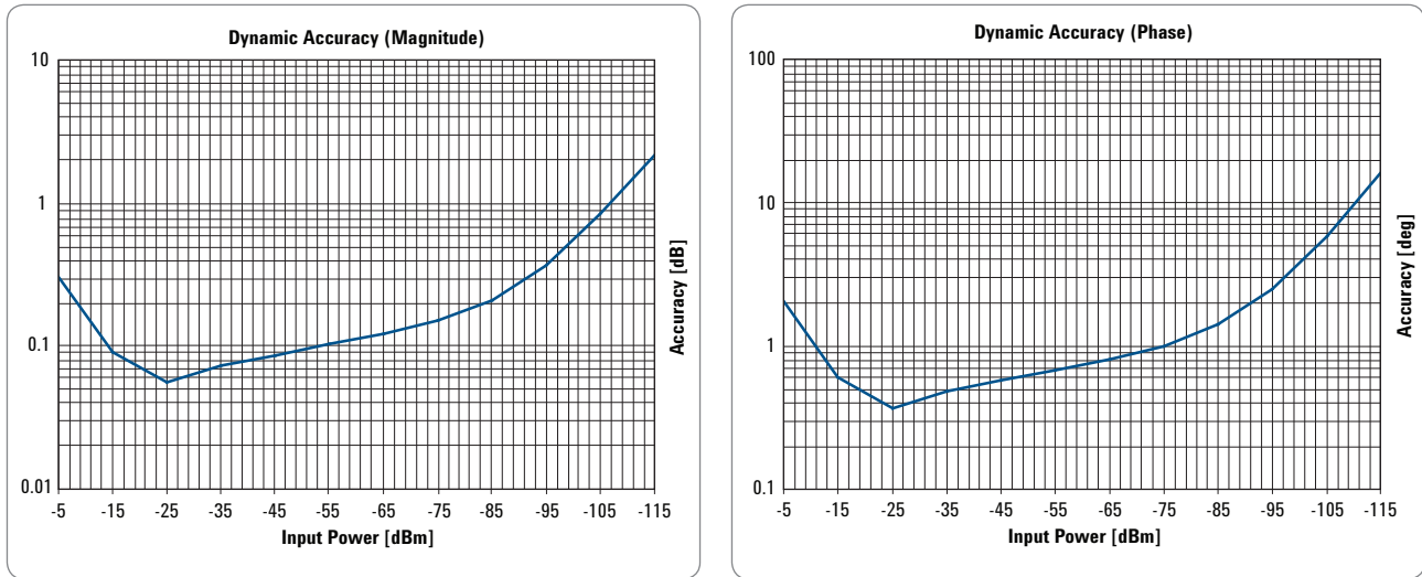
Figure 20. Dynamic Accuracy
