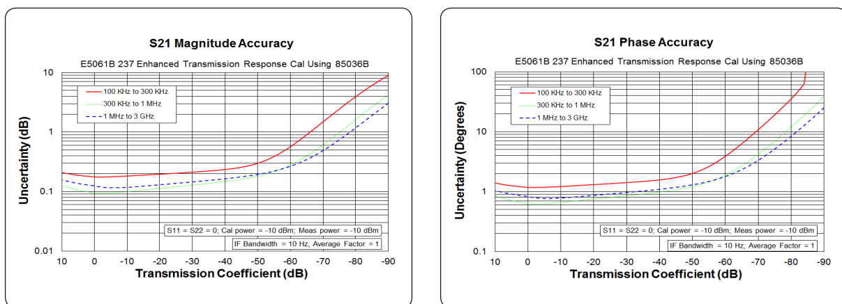
Figure 15. Transmission uncertainty (specification)
