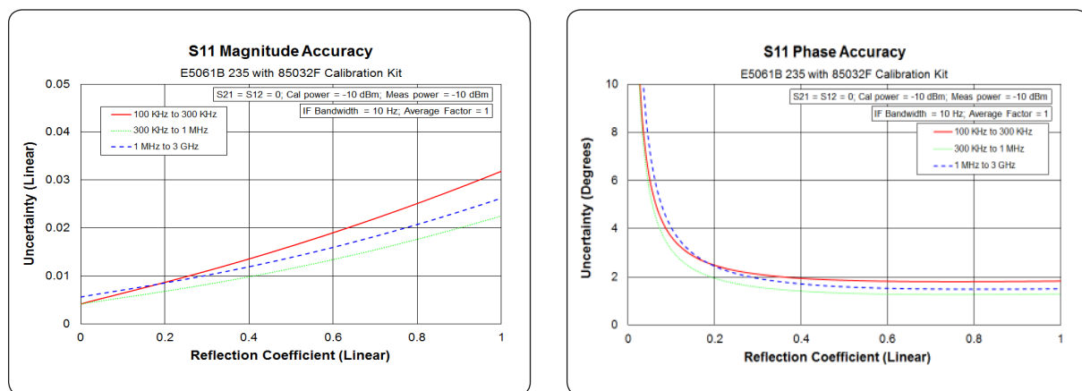
Figure 10. Reflection uncertainty (specification)
