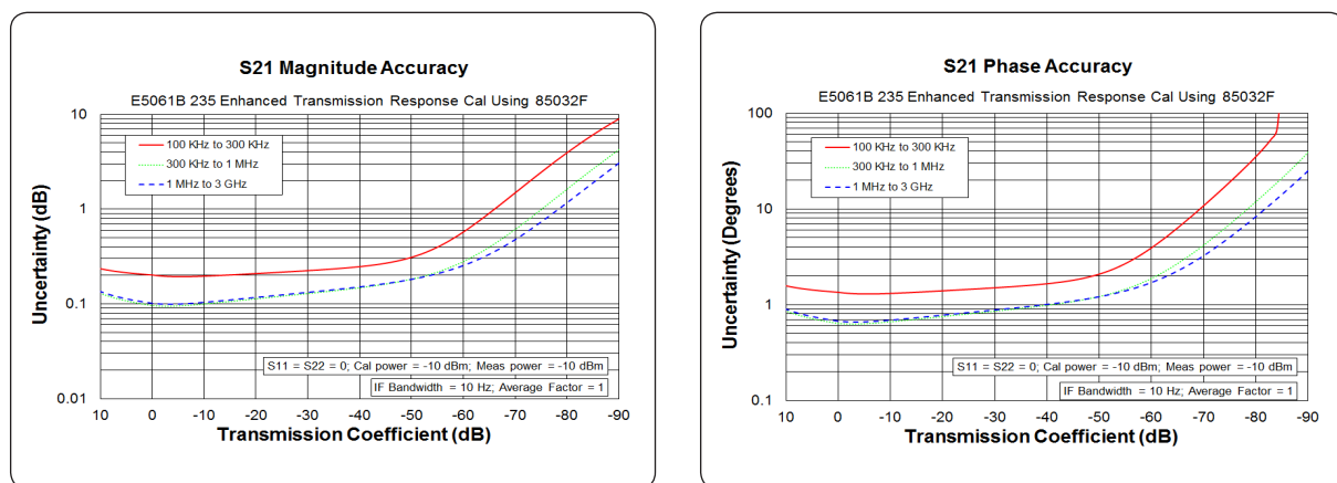
Figure 9. Transmission uncertainty (specification)
