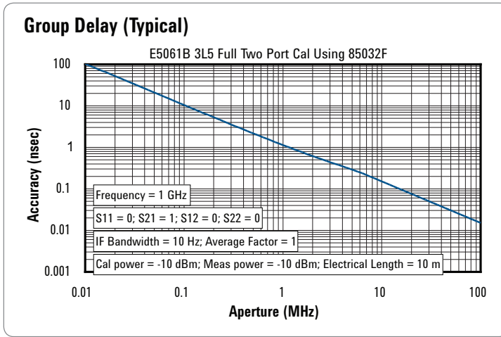
Figure 19. Group delay (typical)
