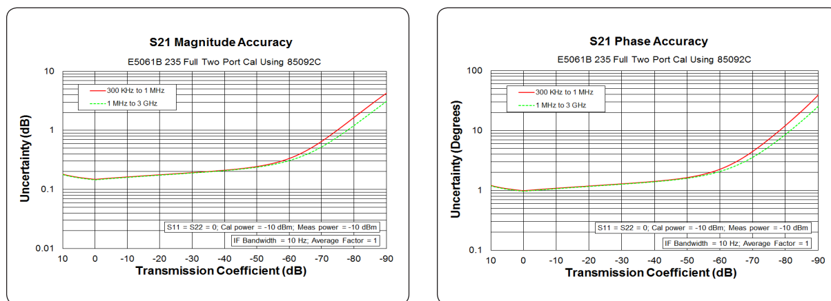
Figure 11. Transmission uncertainty (specification)
