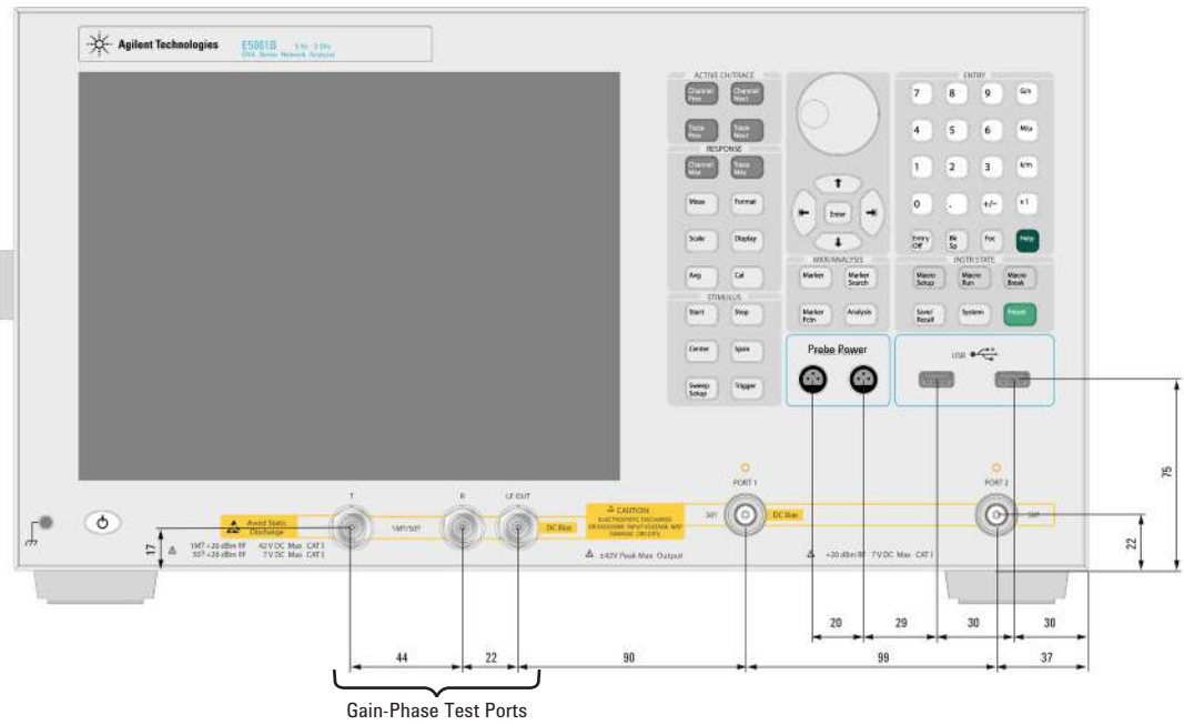
Figure 21. Dimensions (front view, in millimeters) 1
