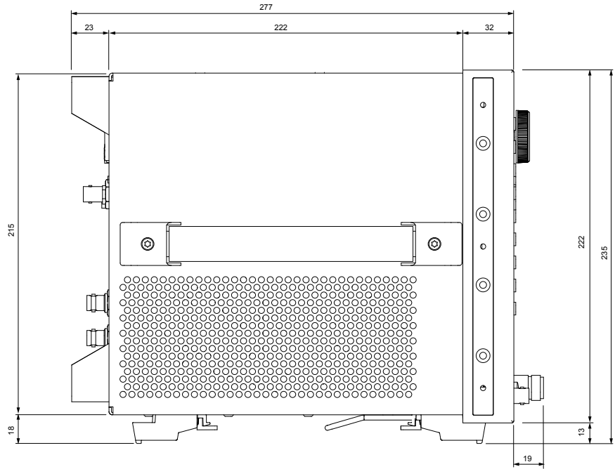
Figure 23. Dimensions (side view, in millimeters)
