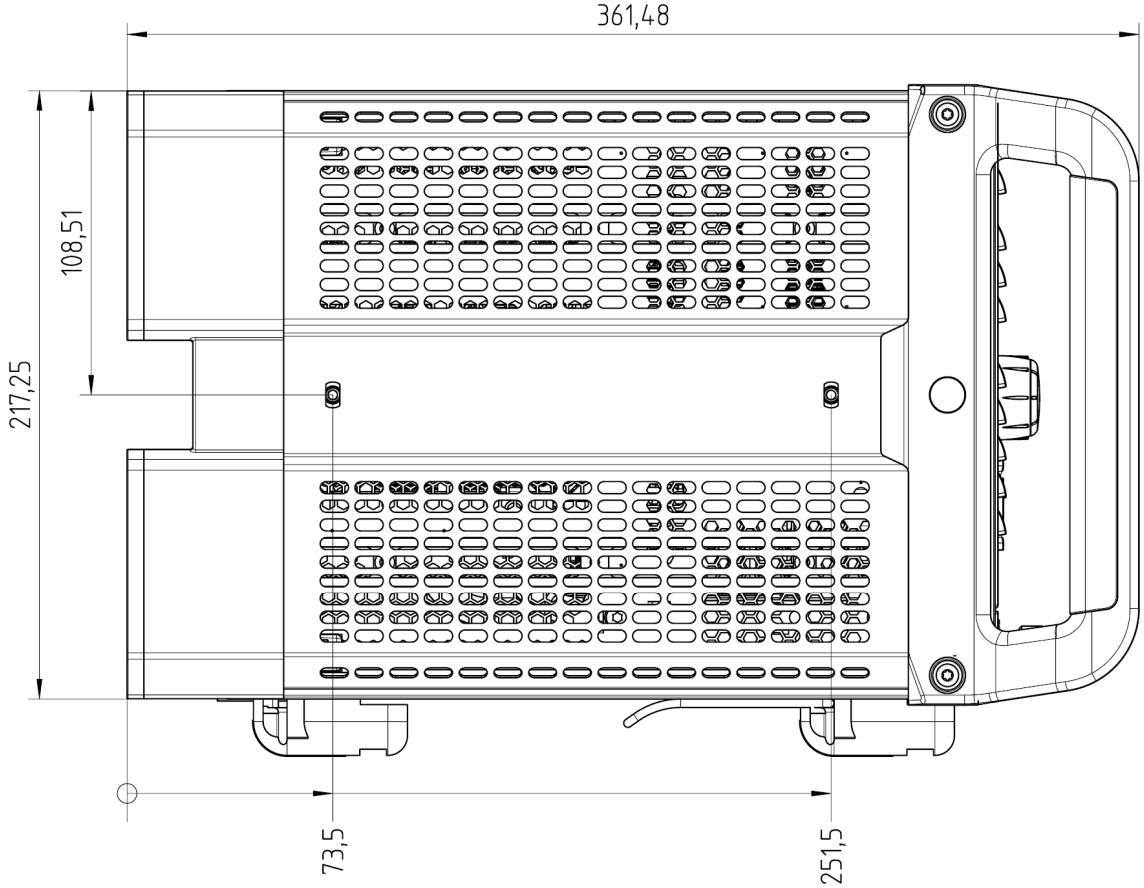
Side view of the R&S ® ZNB.
