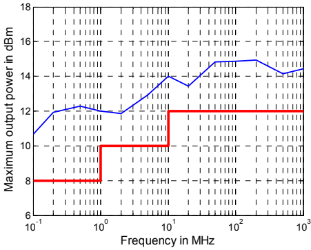
Maximum output power in dBm versus frequency for the R&S ® ZNB20.
