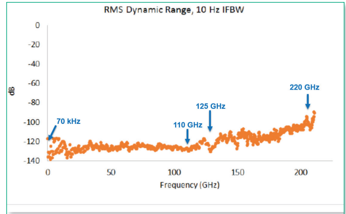
Dynamic Range of VectorStar ME7838G System at the 0.6 mm Test Port from 70 kHz to 220 GHz
