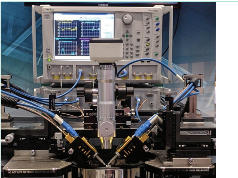
Anritsu's VectorStar ME7838G Broadband System Integrated into an On-Wafer Probe Station
