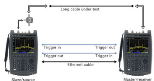
Measure long, lossy cables using ERTA
