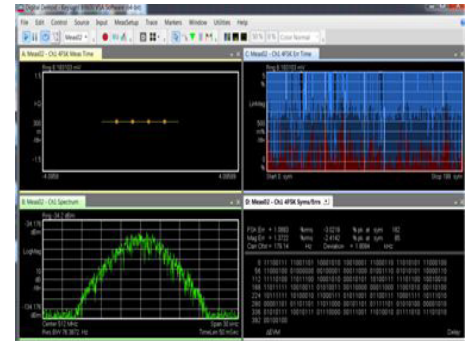
Public safety transmitting signal quality test – P25 C4FM demodulation with FieldFox
