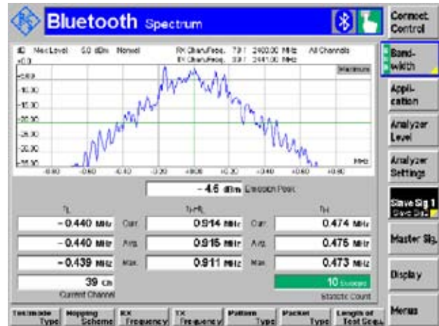
20 dB bandwidth measurement
