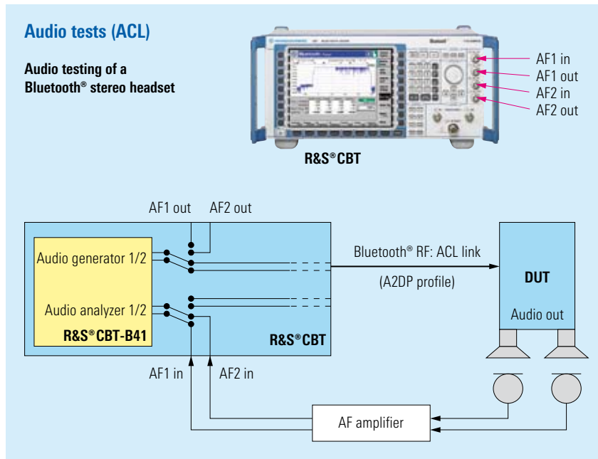
Audio measurement of a stereo headset using the A2DP profile
