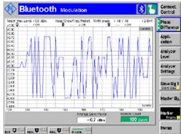
Phase difference characteristic of an EDR packet
