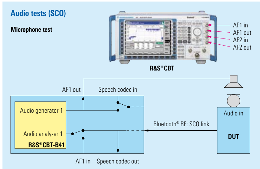
Audio measurement of a DUT microphone with the R&S® CBT-B41 option
