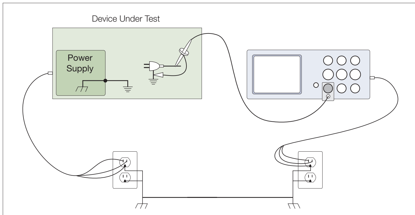
Figure 2. Single-ended voltage measurement on ground-referenced test point.
