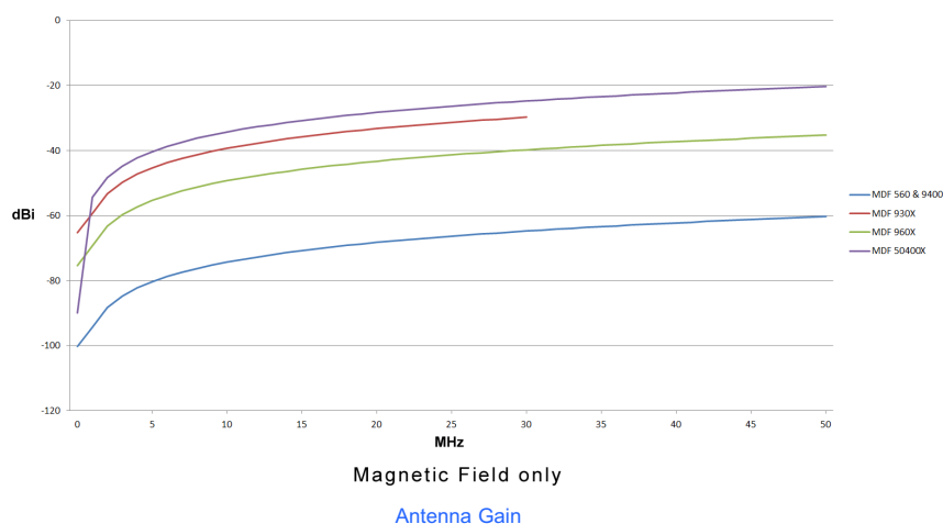
Antenna Gain
