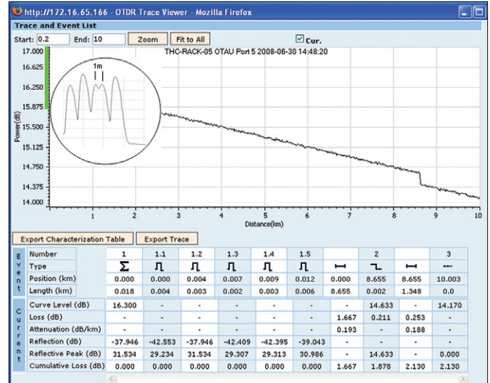
Figure 2. High-resolution view of a fiber link
