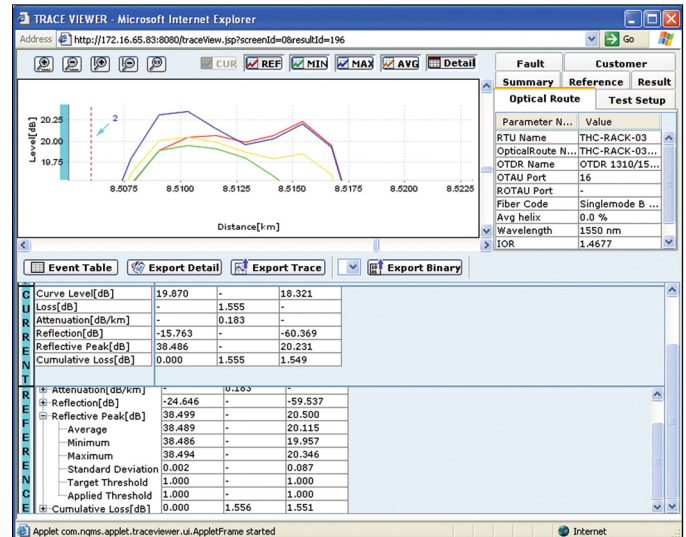
Figure 3. Learning functions acquire multiple traces as part of the reference trace
