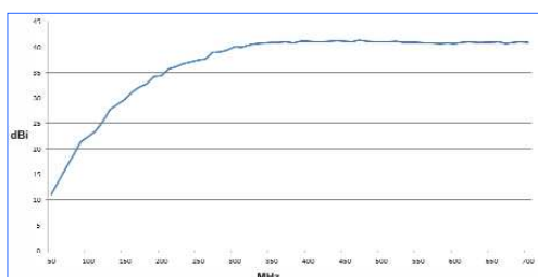
Gain Diagram BicoLOG 5070 X
