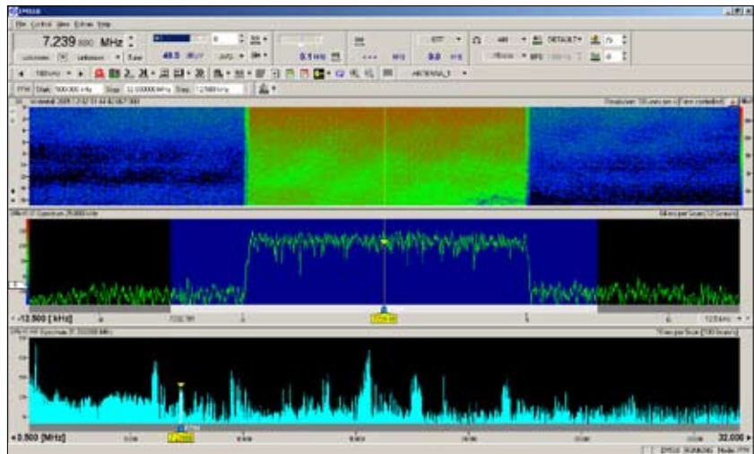
IF spectrum (zoomed) for measurements
