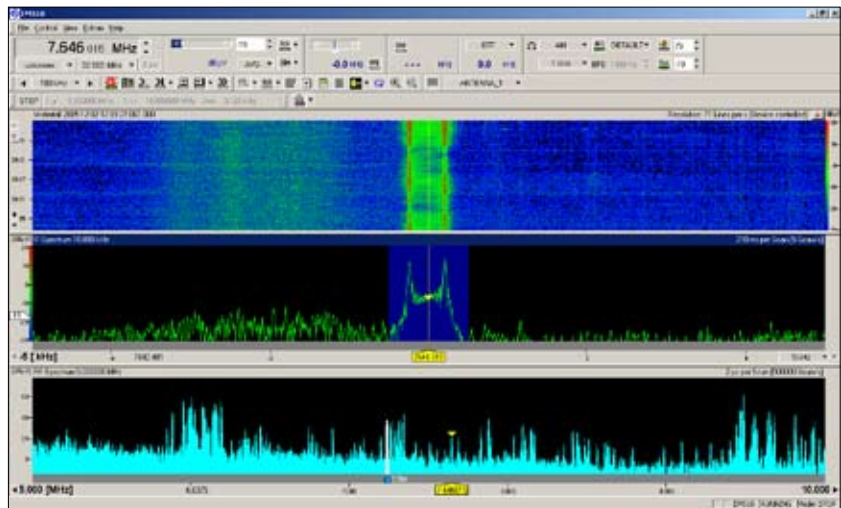
FSK transmission
