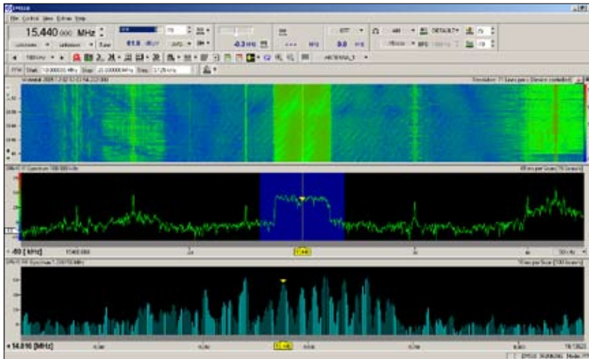
Reception of a digital radio mondial (DRM) signal
