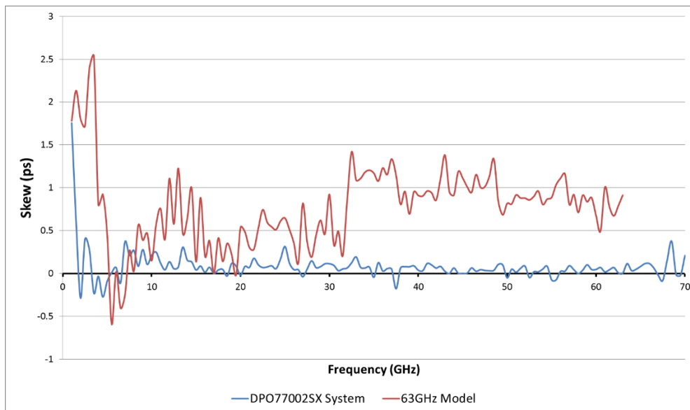
Figure 7: DPO70000SX system shows lower channel-to-channel skew variation over its full frequency range than other vendor's monolithic instrument.
