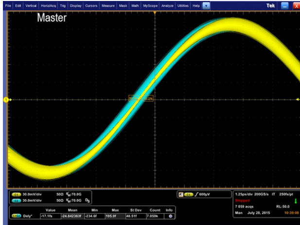
Figure 6: 65 GHz sinewave capture on two ATI channels illustrates inherently high channel-to-channel skew stability.
