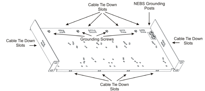
1U Rack Mount Shelf
